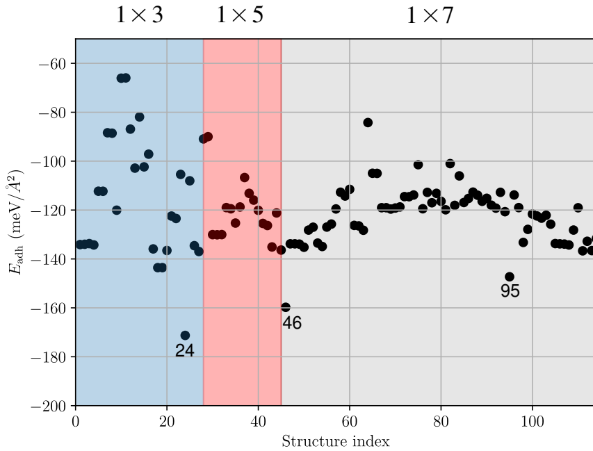
Figure V.7: Adhesion energies ( E_{\text{adh}} ) for all 114 stable phases determined using the USPEX code. All structures were relaxed until forces were below 0.02 \text{ eV}/\text{\AA} . The blue, red, and gray regions represent the structures with 1 \times 3 , 1 \times 5 , and 1 \times 7 supercell substrates, respectively.
