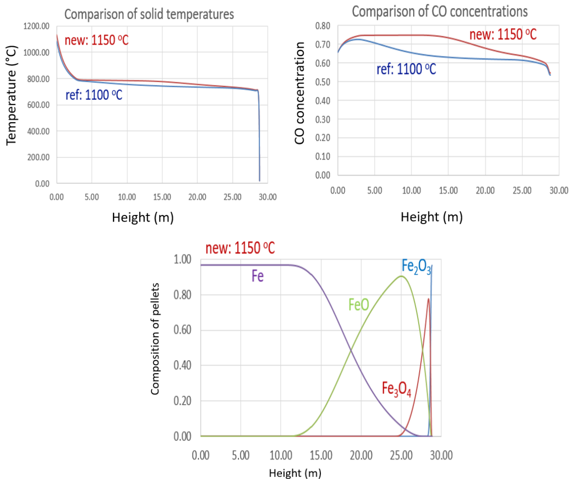
Figure 63. Sensitivity analysis on the effect of inlet gas temperature
