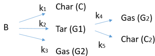
Figure 29. Kinetic mechanism of biomass decomposition into two steps
