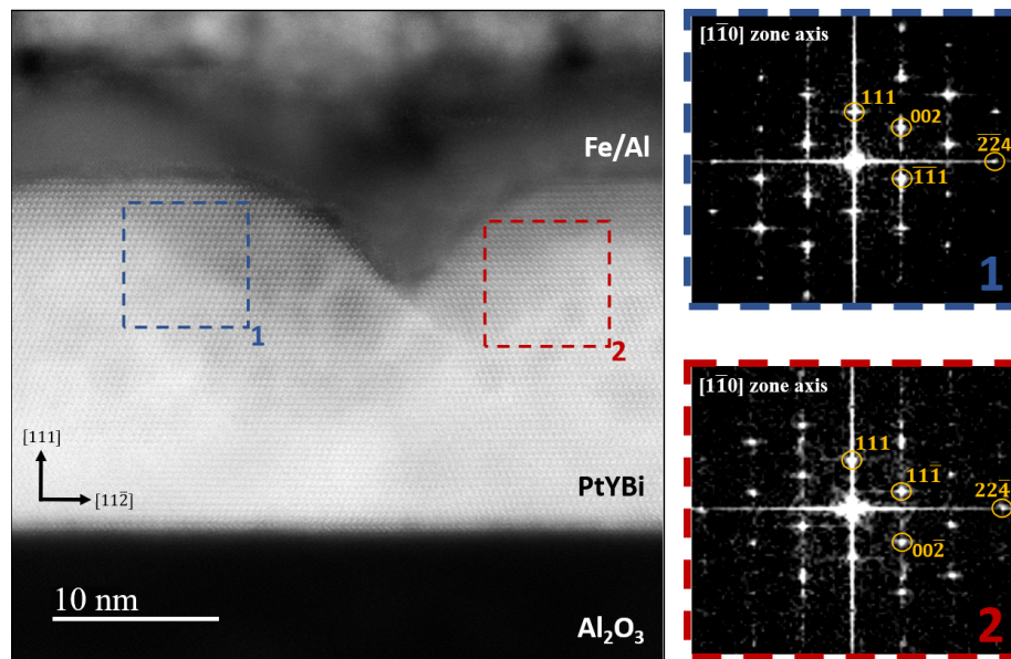
FIGURE 1.41: STEM-HAADF image of \text{Al}_2\text{O}_3/\text{PtYBi}/\text{Fe}/\text{Al} . On the right, diffraction patterns of the blue and red squared frames allowing to distinguish the presence of domains.
