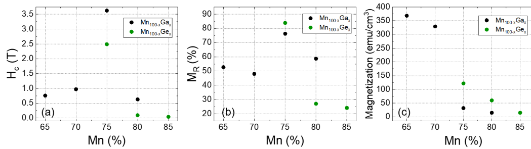
FIGURE 2.21: Comparison of the coercive field (a), magnetization remanence (b) and magnetization (c) extracted as a function of Mn content between Mn 100-x Ga x (in black) and Mn 100-x Ge x (in green) series.
