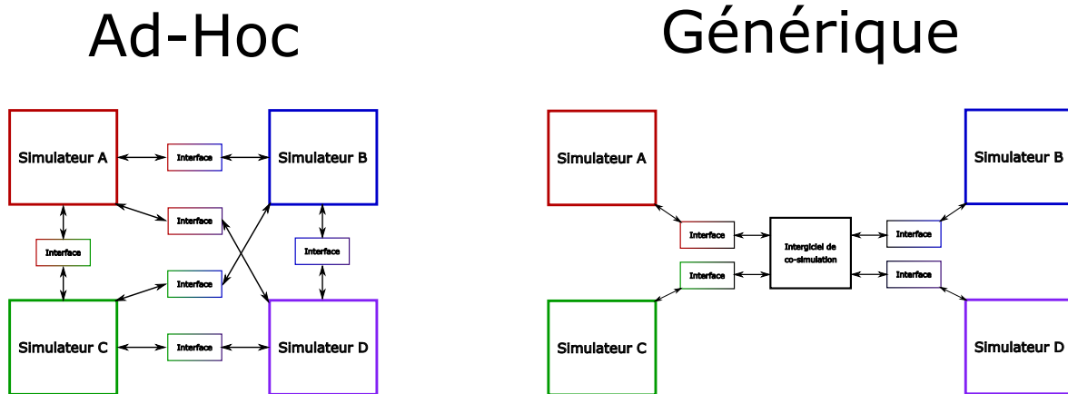
FIGURE 2.6 – Approche de co-simulation ad hoc et générique [?]
