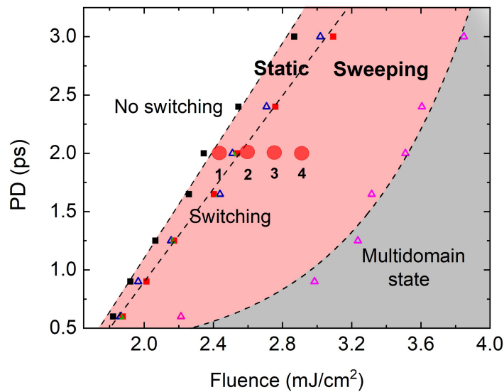
FIGURE 3.7 – Magnetization state diagram as a function of the laser fluence and the pulse duration (PD), obtained with left circularly polarized \sigma^- laser in both static and sweeping mode. For a given pulse duration, the black and red solid squares indicate, respectively, the critical fluence for switching and minimum fluence required for multidomain-formation in static mode. In the case of sweeping mode, two fluences are indicated by blue and pink hollow triangle, respectively.
