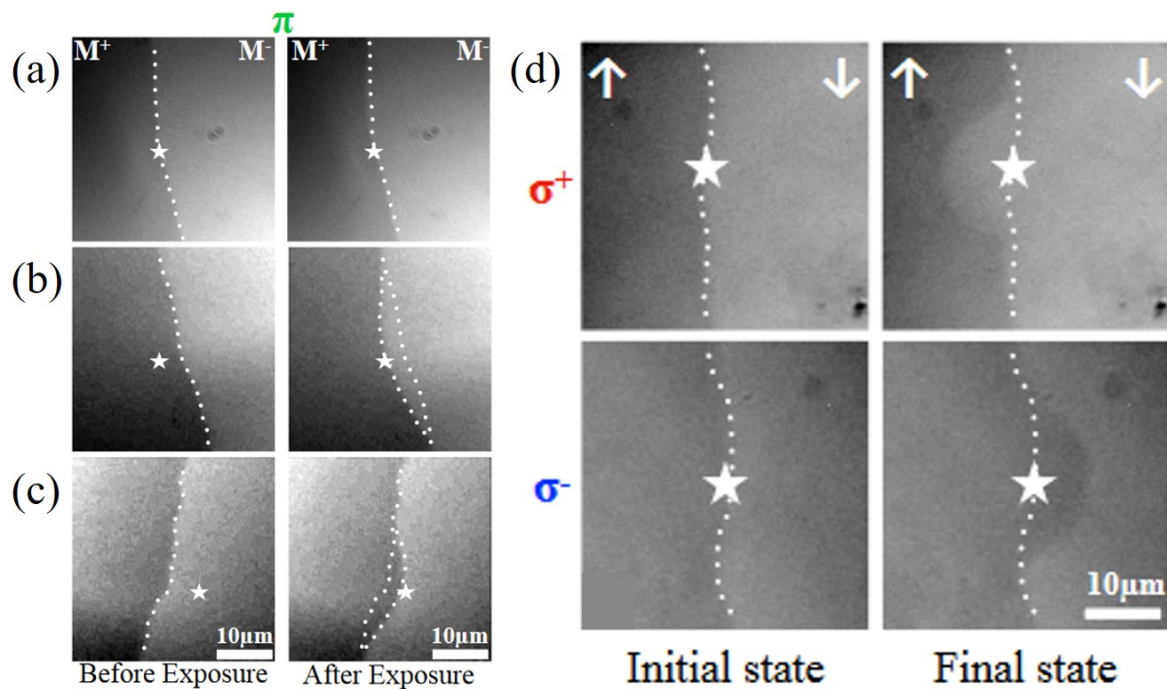
FIGURE 3.12 – (a) and (b) MOKE images of a DW in Co/Pt multilayers exposed to 40-fs linearly polarized ( L ) laser pulses with a fluence of 7 \text{ mJ/cm}^2 . The laser beam spot (star) is (a) on the DW and off-centered in (b) and (c). The DW moves towards the center of the beam which is the hottest regions 107 . (d) MOKE images taken before and after exposure centered on DW and with a fluence below the switching threshold 106 .
