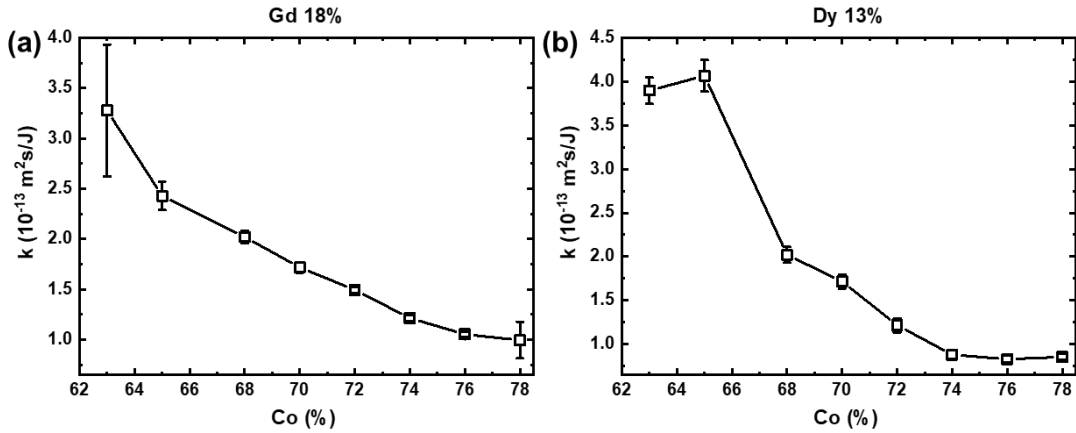
FIGURE 4.17 – The slope k as a function of Co concentration in (a) \text{Gd}_{18}\text{DyCo} alloys and (b) \text{GdDy}_{13}\text{Co} .
