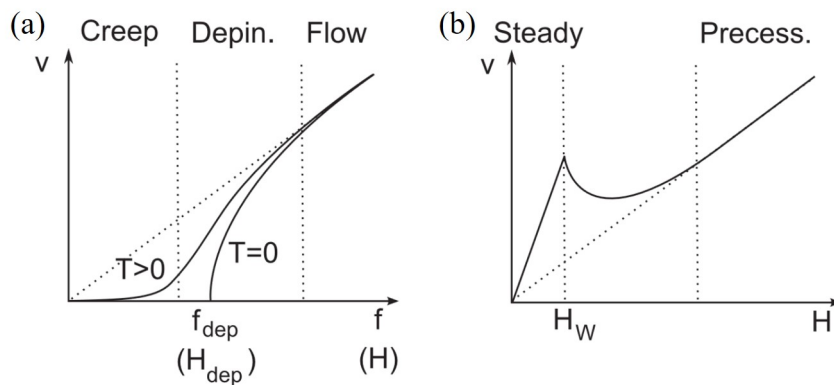
FIGURE 3.9 – (a) Theoretical variation of the velocity v of a DW in a 2D weakly disordered medium submitted to magnetic field at zero and finite temperature T . The creep, depinning and flow regimes are labeled. (b) Regimes of DW flow motion in an ideal ferromagnetic film without pinning. The steady and precessional linear flow regimes are separated by an intermediate regime which begins at the Walker field H_W . 156
