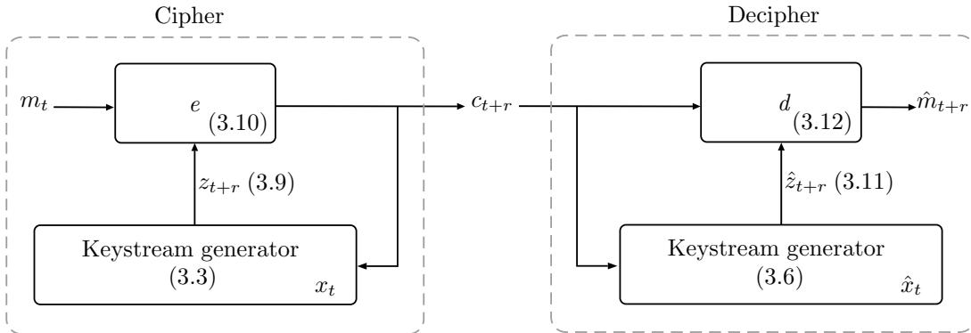
Figure 3.9: Flat LPV-based Self-Synchronizing Stream Ciphers block diagram.
