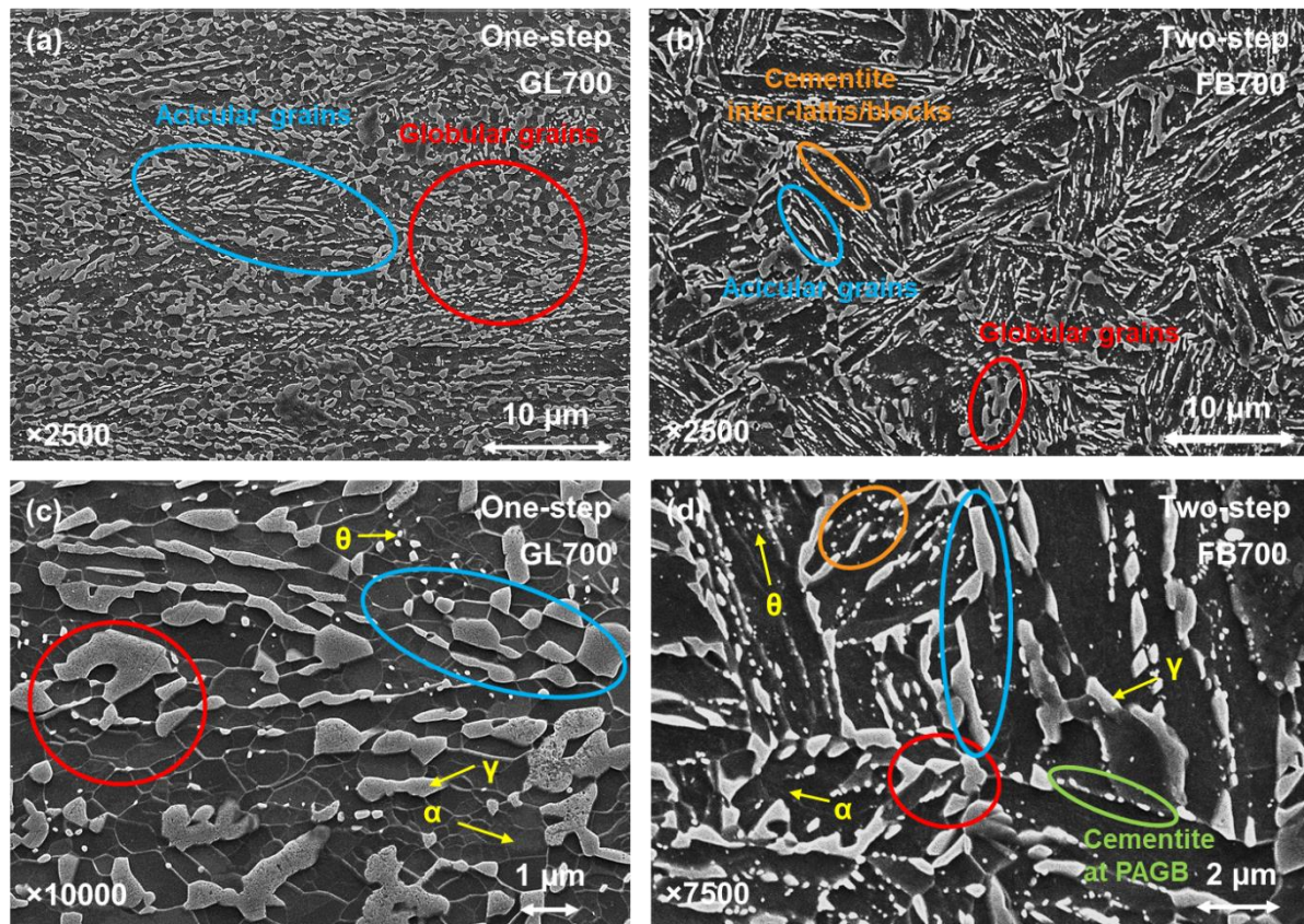
Figure 69: SEM micrographs of globular and fibrous microstructures annealed at 700°C. (a) GL700 magnified at \times 2500 . (b) FB700 magnified at \times 2500 . (c) GL700 magnified at \times 10000 . (d) FB700 magnified at \times 7500 . Ferrite appears in dark grey, austenite in light grey, cementite in white particles.
