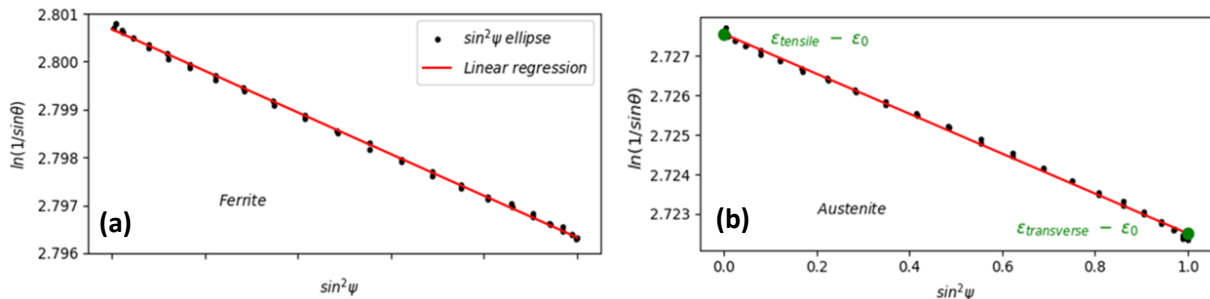
Figure 85: Example of measured strains for the (a) \{211\}_\alpha and (b) \{311\}_\gamma planes as a function of \sin^2\psi in the elastic regime. Each dot (black) corresponds to a measurement in a 4^\circ sector of the Debye-Scherrer. The Y-axis \ln(1/\sin\theta_B^{peak}) is linked to the strain in the \phi, \psi direction by Equation: ( III-4 ). A linear interpolation (red curve) is represented for the sake of readability. The green dots are linked to the elastic strain measured in the tensile and transverse directions, respectively [187].
