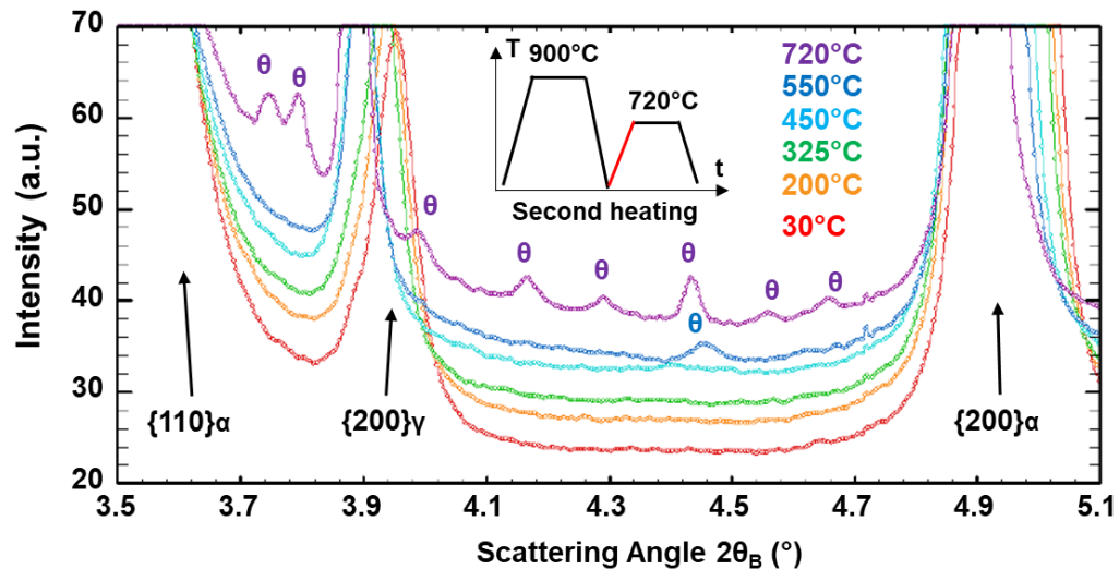
Figure 48: Evolution of diffractograms during the heating step of intercritical annealing of FB720 steel. The main diffraction peaks are generated by austenite and ferrite. The small peaks appearing above 550°C (dark blue and purple diffractograms) are generated by cementite.
