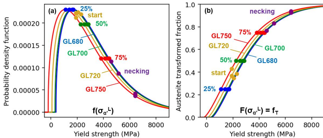
Figure 133: Evolution of the (a) density function and (b) cumulative function for the 4 globular microstructures. Dots have been added at given austenite transformed fraction. (blue: f_T=0.25 ; green: f_T=0.50 ; red: f_T=0.75 ). The yellow and purple points are respectively indicative of the experimental values of f_T at the start of the trial and at the necking onset.
