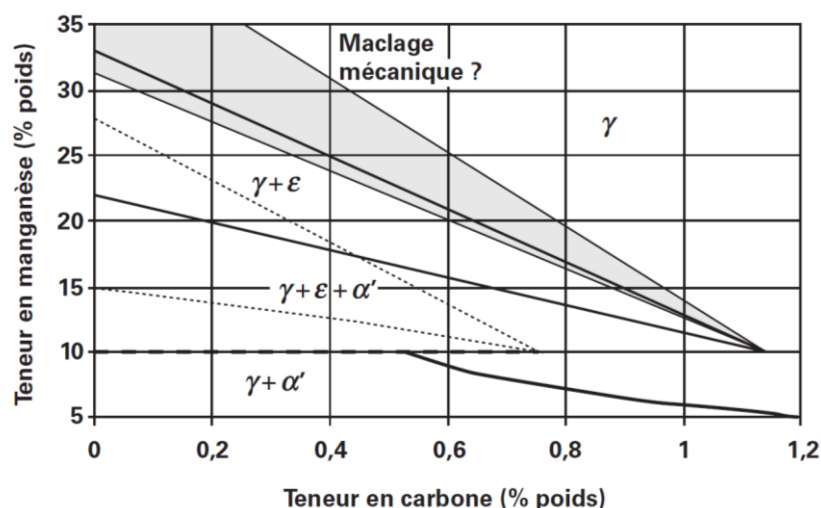
Figure 24: Microstructure of austenitic steels after quenching and deformation at room temperature as a function of carbon and manganese alloying content (wt%) [36], [37].
