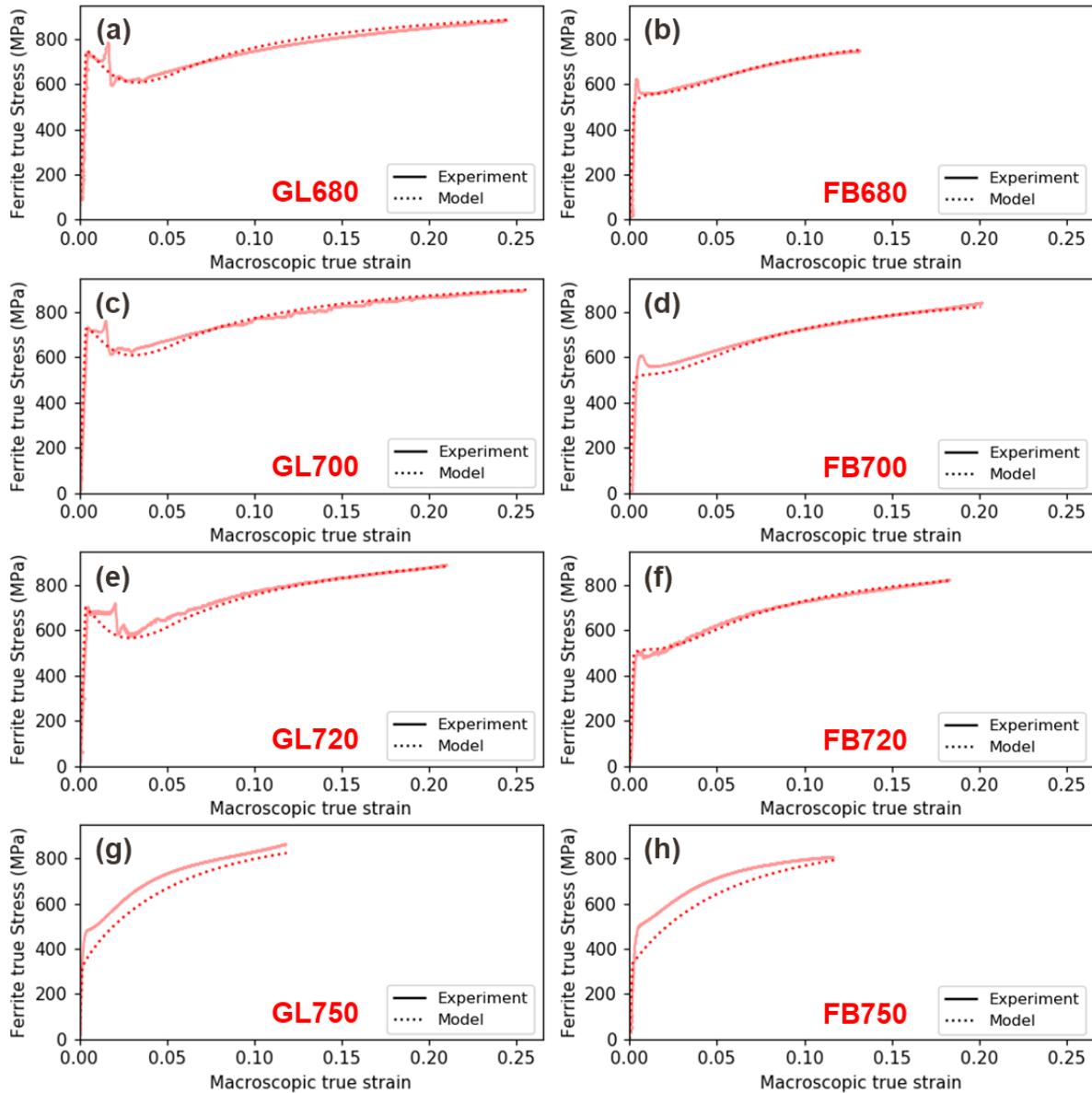
Figure 126: Comparison between the simulated flow stress (dotted line) and the experimental von Mises stress (solid line) in ferrite for (a) GL680, (b) FB680, (c) GL700, (d) FB700, (e) GL720, (f) FB720, (g) GL750, (h) FB750 steels respectively. The stresses in ferrite are plotted as a function of \epsilon_{macro} .
