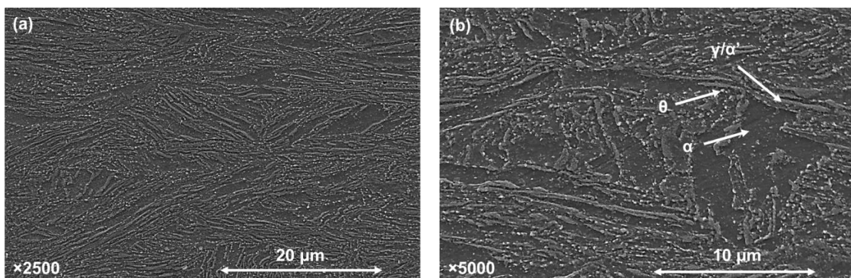
Figure 44: SEM micrographs of the cold-rolled steel (a) at a magnification of \times 2500 and (b) at a magnification of \times 5000 . The rolling direction is horizontal. The black-grey areas correspond to ferrite, while the light-grey areas correspond to austenite-martensite elongated islands and bright areas to cementite particles.
