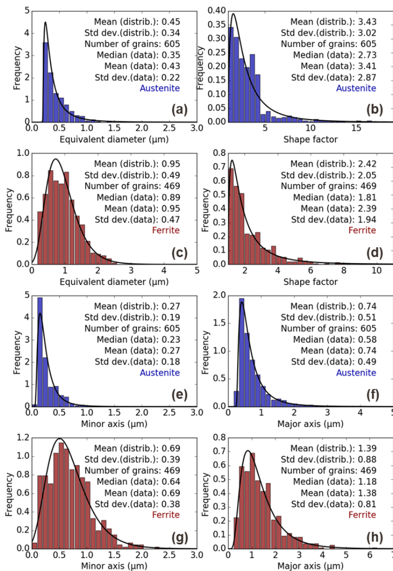
Figure 164: Distributions of (a) and (c) equivalent diameter, (b) and (d) shape factor, (e) and (g) minor axis and (f) and (h) major axis for both (c), (d), (g) and (h) ferrite grains, and (a), (b), (e) and (f) austenite/martensite islands, in the globular microstructure annealed at T_{IA} = 680^{\circ}\text{C} .
