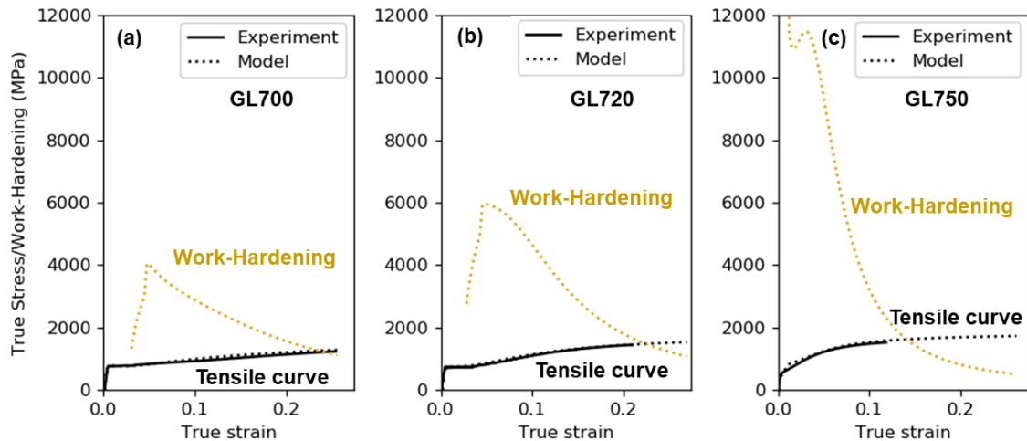
Figure 139: Comparison between the experimental true stress (black solid line), the true stress calculated by the model (black dotted line) and the model work-hardening rate (yellow dotted line).
