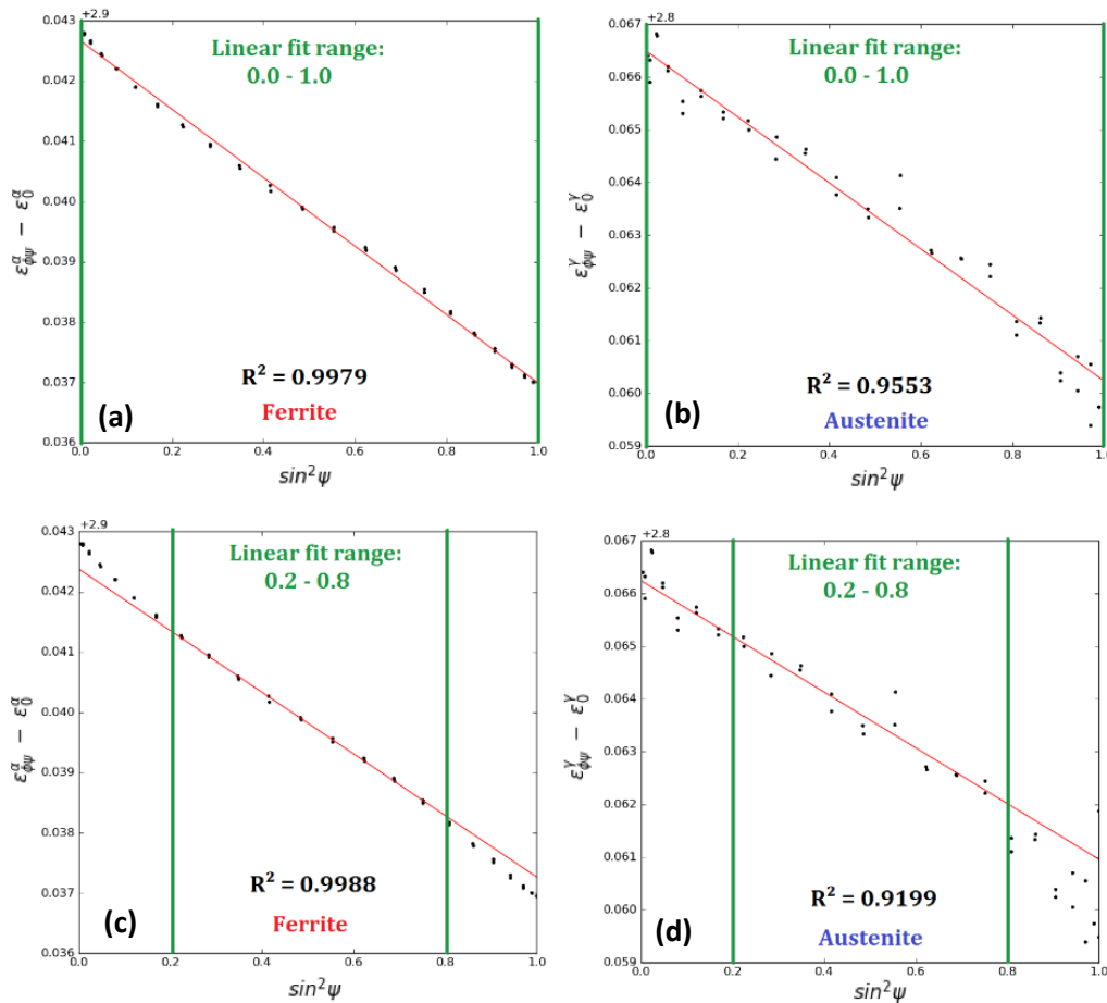
Figure 172: \sin^2\psi ellipse (black dots) obtained on the GL720-001 experiment at the onset of necking (diffraction image n°4734) for ferrite (a and c) and austenite (b and d). The red line in each subplot corresponds to the results of the linear regression over the \sin^2\psi range indicated in green. The coefficient of determination R^2 of each linear regression is indicated.
