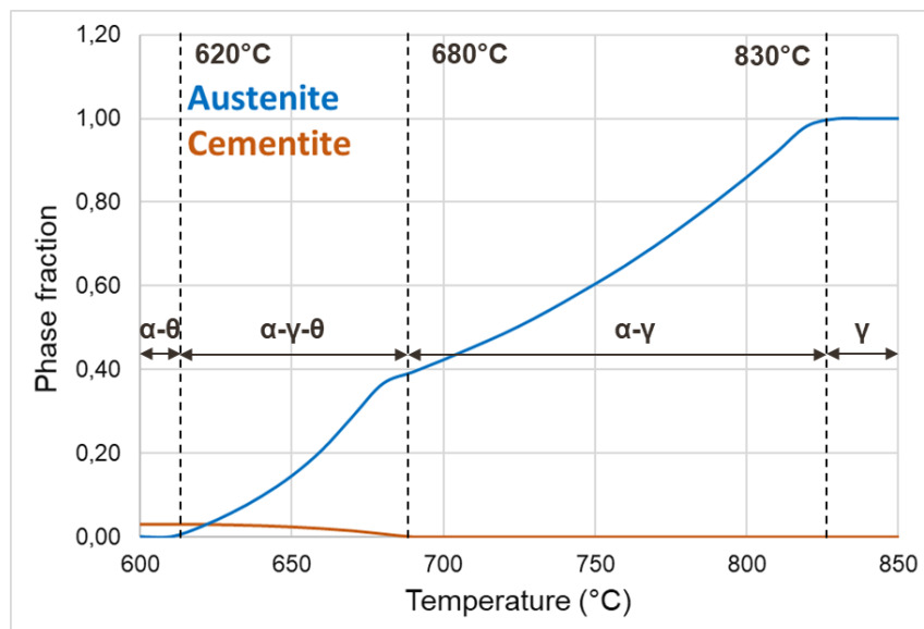
Figure 42: Austenite (blue) and cementite (orange) phase fractions expected at equilibrium as a function of the intercritical annealing temperature. Thermodynamical equilibrium calculations were conducted with CEQCSI software.
