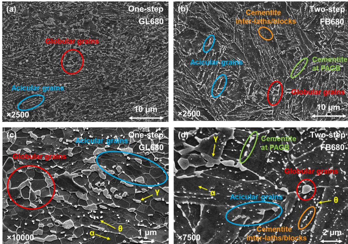
Figure 68: SEM micrographs of globular and fibrous microstructures annealed at 680°C. (a) GL680 magnified at \times 2500 . (b) FB680 magnified at \times 2500 . (c) GL680 magnified at \times 10000 . (d) FB680 magnified at \times 7500 . Ferrite appears in dark grey, austenite in light grey, cementite in white particles.
