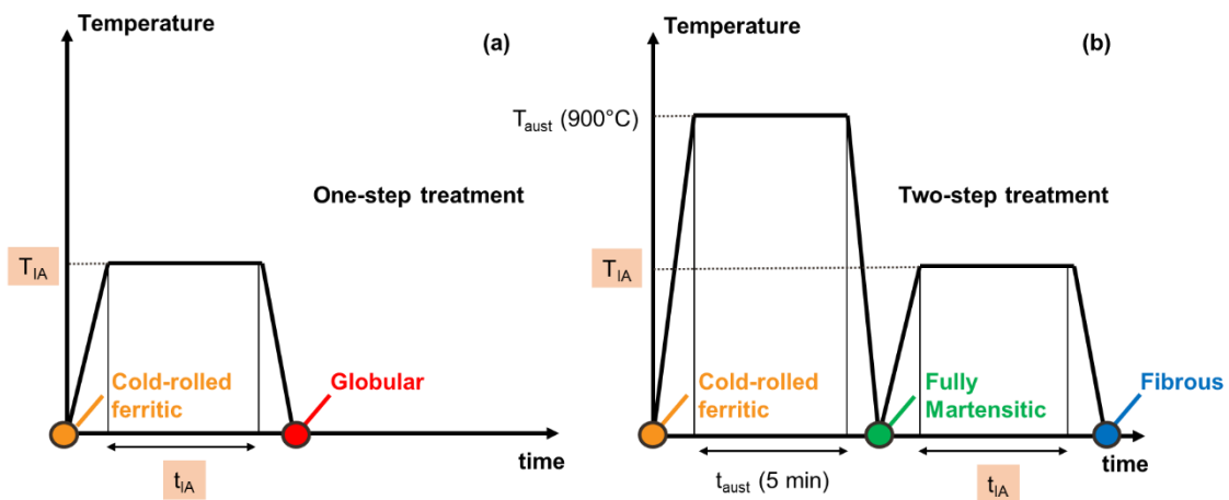
Figure 43: Schematic representations of the thermal treatments applied on the studied steel. (a) One step annealing to obtain globular cold-rolled UFG steels. (b) Two-step annealing to obtain fibrous ART steels. Values of parameters highlighted in orange can be found in Table 2. The initial microstructure state before all thermal treatments is cold-rolled ferrite-cementite-martensite.
