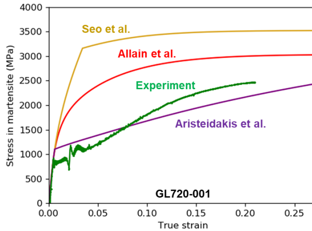
Figure 124: Comparison between the experimental von Mises stress determined in martensite for GL720 steel, and the predictions of the models of Seo et al. [126], Aristeidakis et al., Allain et al. [212] respectively.
