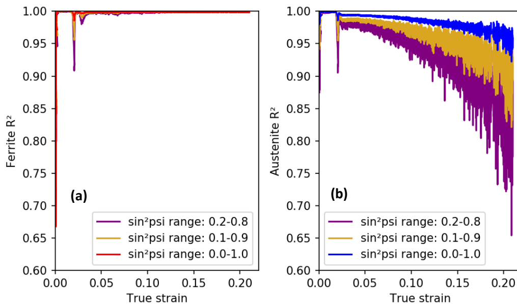
Figure 174: Effect of the \sin^2\psi range used for linear fit on the coefficient of determination R^2 in ferrite (a) and austenite (b) of the GL720-001 experiment. The R^2 curves in red in (a) and blue in (b) are R^2 values obtained after linear fitting over the whole \sin^2\psi range. In gold are the curves obtained after a linear fit over 0.1-0.9 \sin^2\psi range, and in purple the ones obtained over 0.2-0.8 \sin^2\psi range.
