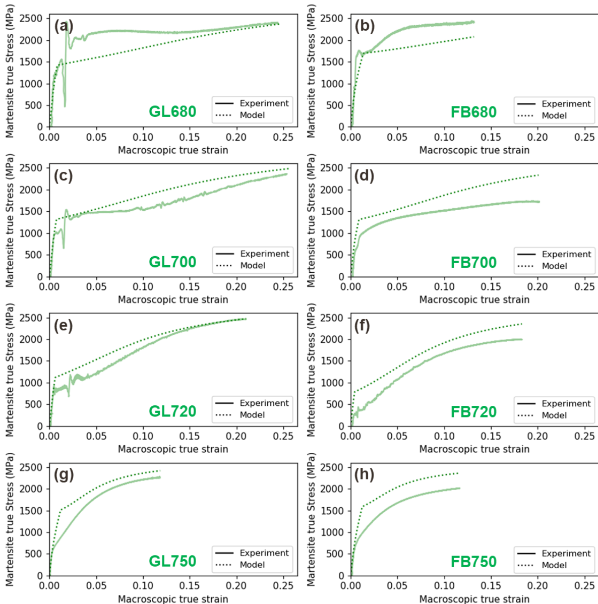
Figure 136: Comparison between the simulated flow stress (dotted line) and the experimental von Mises stress (solid line) in martensite for (a) GL680, (b) FB680, (c) GL700, (d) FB700, (e) GL720, (f) FB720, (g) GL750, (h) FB750 Steels. The stresses in martensite are shown as a function of \epsilon_{\text{macro}} .
