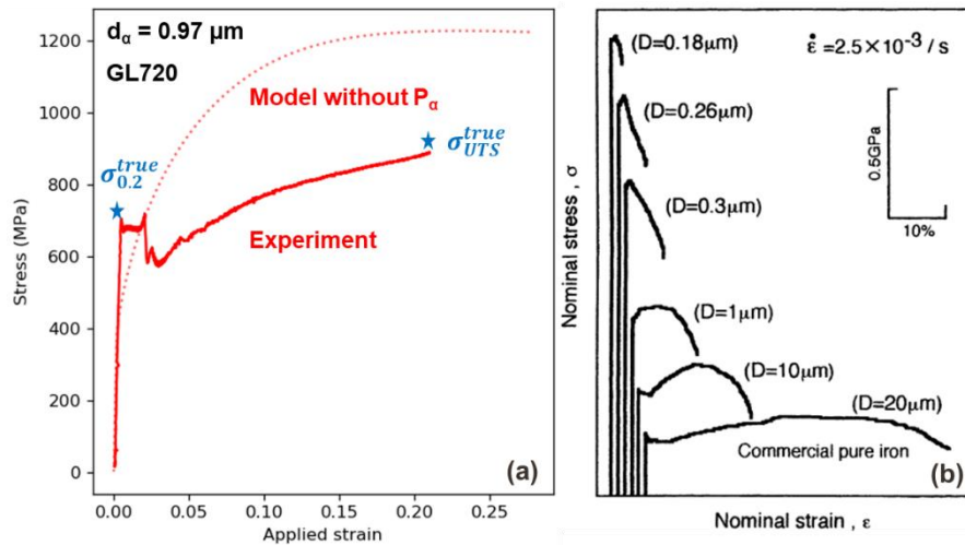
Figure 123: (a) Comparison between the experimental von Mises stress determined in ferrite for GL720 steel, and the predictions of the original model of Bouaziz et al. [14], which does not account for the P_\alpha coefficient. (b) Tensile curves of shoot-pinned IF steels by Takaki et al. [205]. The grain size of ferrite is indicated above the corresponding curve. In (a), the blue star corresponds to value of true stress at yielding and necking onset determined with grain size sensitive equation given by Takaki et al. [205].
