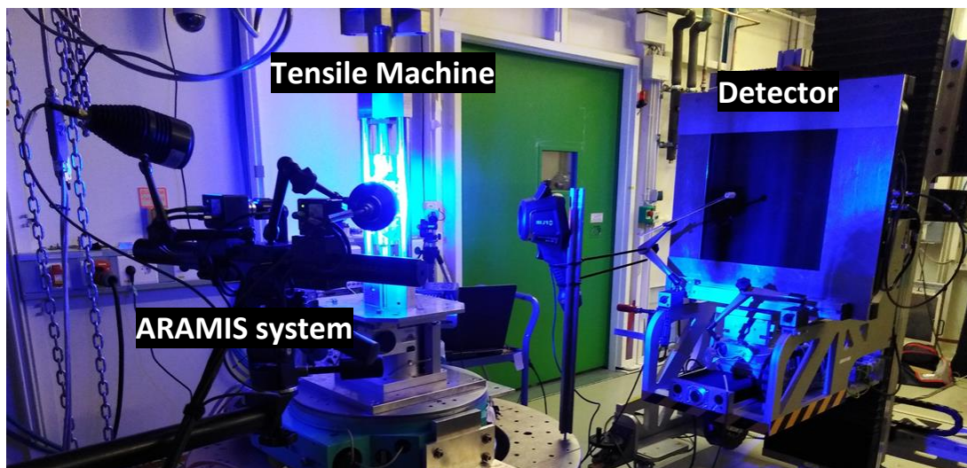
Figure 78: Picture of an experiment conducted at DESY synchrotron on P07 beamline (Nov. 2020). From left to right: the incoming X-Ray beam produced by the synchrotron ring comes from the left side of the photo (not visible). Aramis stereographic system is composed of two cameras and two blue led lamps. Cameras are placed 34 cm from the tensile specimen. The sample placed in a tensile tester is illuminated by the blue led lamps (appears in white/light blue). The Perkin Elmer 2D flat detector which acquires diffraction pattern appears on the right of the image.
