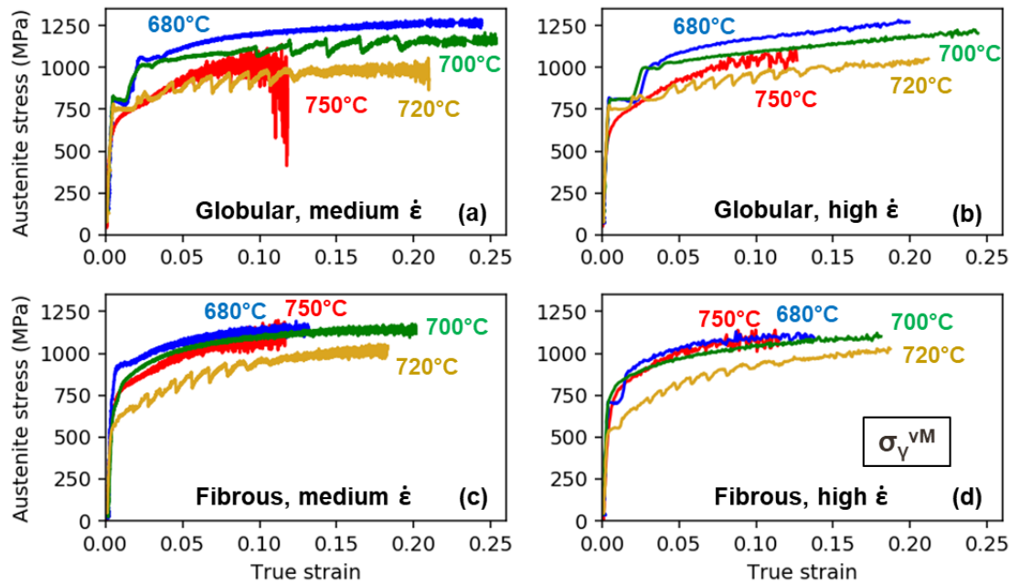
Figure 104: Austenite von Mises stress as a function of macroscopic true strain for the 16 experiments at the two higher strain rates: (a) globular, medium \dot{\epsilon} ; (b) globular, high \dot{\epsilon} ; (c) fibrous, medium \dot{\epsilon} ; (d) fibrous, high \dot{\epsilon} .
