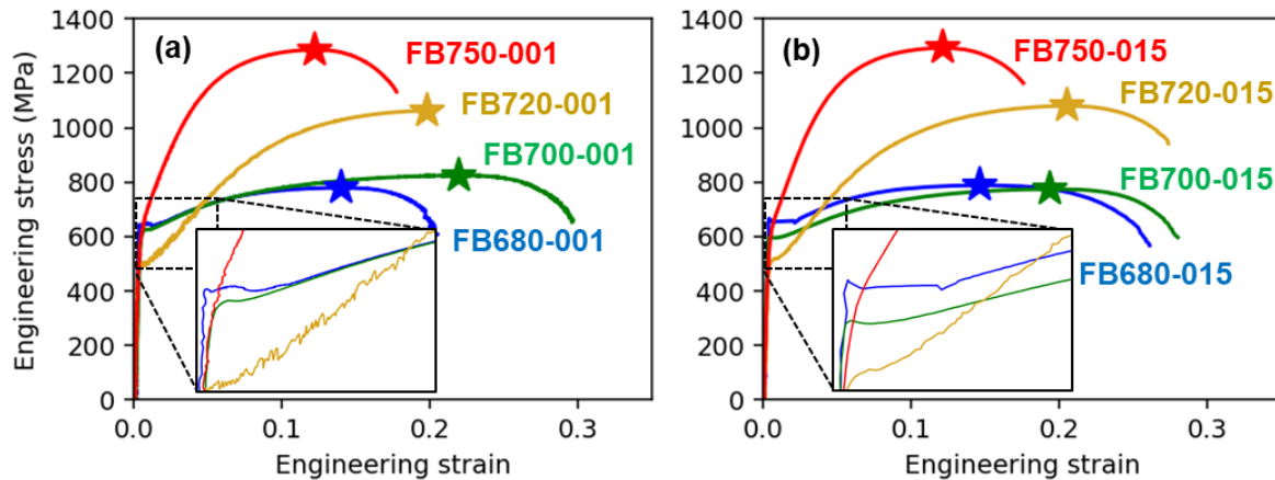
Figure 89: Engineering tensile curves of samples with fibrous microstructures at (a) the medium and (b) high strain rates. The stars correspond to the onset of necking.
