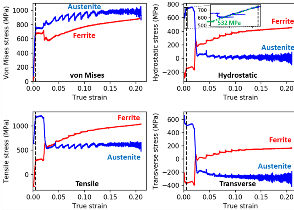
Figure 93: Evolution of stress tensor components in ferrite (red) and austenite (blue) obtained during the GL720-001 experiment: (a) von Mises stress \sigma_{VM} ; (b) hydrostatic pressure \sigma_h ; (c) stress in tensile direction \sigma_{RD} ; (d) stress in transverse direction \sigma_{TD} . The vertical dotted black line corresponds to the onset of yielding. The curves are cut at the necking onset. The measurement error on stress is around 25 MPa. In (b), a magnification of the austenite hydrostatic stress in the elastic domain highlights how the stresses are calibrated to respect the chosen initial hydrostatic values in both phases.
