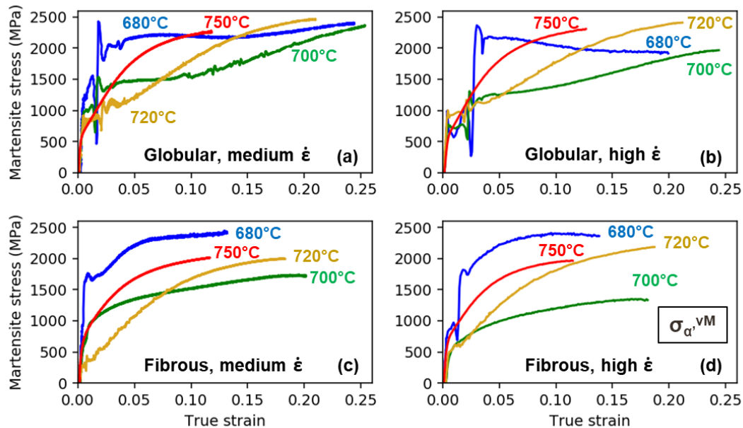
Figure 106: Martensite von Mises stress as a function of macroscopic true strain for the 16 experiments at the two higher strain rates: (a) globular, medium \dot{\epsilon} ; (b) globular, high \dot{\epsilon} ; (c) fibrous, medium \dot{\epsilon} ; (d) fibrous, high \dot{\epsilon} .
