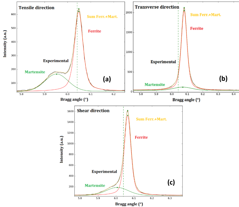
Figure 86: Deconvolution of ferrite (red) and martensite (green) \{211\} peaks family from the experimental peak (black) obtained after integration of diffraction pattern (a) in the tensile direction ( 0^\circ ), (b) in the transverse direction ( 90^\circ ) and (c) in the diagonal direction ( 45^\circ ) at the onset of necking. The curves in yellow are the sum of martensite and ferrite simulated peaks and must be compared to the experimental curve in black. The results are extracted from GL720-001 experiment.
