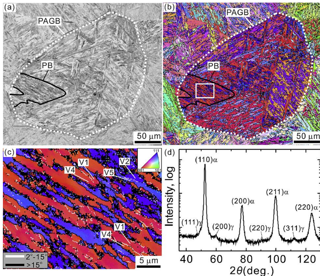
Figure 25: Martensite laths found in an as-quenched steel (Fe/0.3C/2Mn/1.5Si) observed in (a) an OM micrograph and (b) an EBSD orientation map. PAGB corresponds to the prior austenite grain boundary, PB corresponds to a packet boundary. (c) is a zoom from the white rectangle in the (b) map, where low and high angle boundaries are indicated. (d) is the X-ray diffraction profile of the specimen [7].
