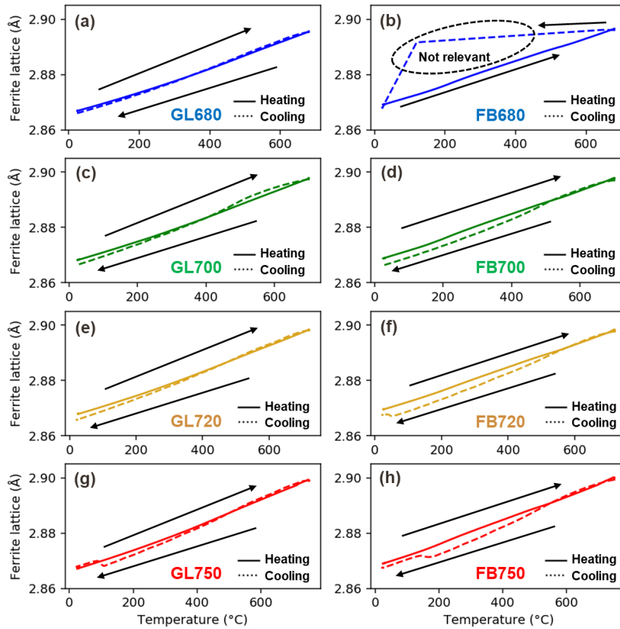
Figure 55: Evolution of the ferrite lattice parameter as a function of temperature for the 8 considered intercritical annealing experiments: (a) GL680, (b) FB680, (c) GL700, (d) FB700, (e) GL720, (f) FB720, (g) GL750 and (h) FB750. Dashed line corresponds to the cooling step, while continuous line corresponds to the soaking and heating steps. The cooling sequence of the FB680 has not been conducted with the relevant acquisition rate, as a consequence, the measurements may not be physically relevant.
