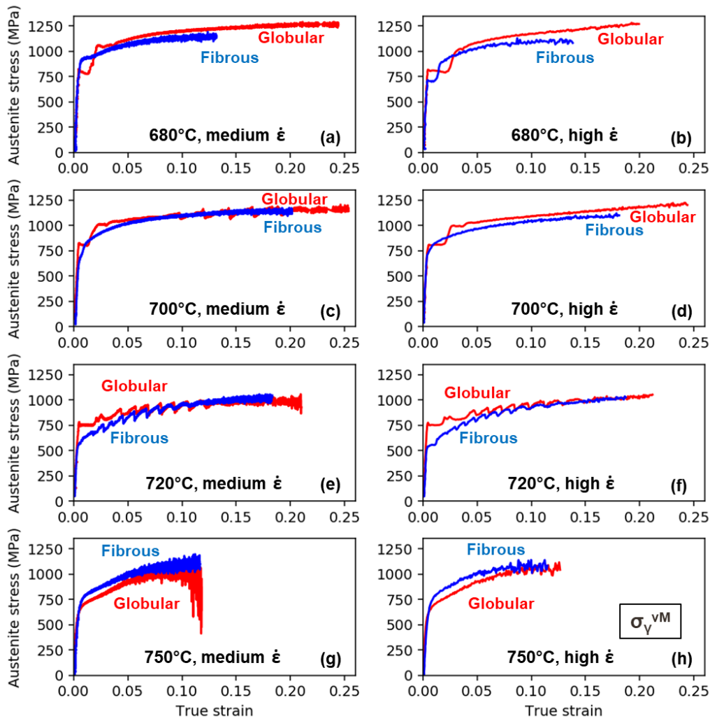
Figure 110: Austenite von Mises stress as a function of macroscopic true strain for the 16 experiments at the two higher strain rates: (a) T_{IA} = 680^{\circ}\text{C} , medium \dot{\epsilon} ; (b) T_{IA} = 680^{\circ}\text{C} , high \dot{\epsilon} ; (c) T_{IA} = 700^{\circ}\text{C} , medium \dot{\epsilon} ; (d) T_{IA} = 700^{\circ}\text{C} , high \dot{\epsilon} ; (e) T_{IA} = 720^{\circ}\text{C} , medium \dot{\epsilon} ; (f) T_{IA} = 720^{\circ}\text{C} , high \dot{\epsilon} ; (g) T_{IA} = 750^{\circ}\text{C} , medium \dot{\epsilon} ; (h) T_{IA} = 750^{\circ}\text{C} , high \dot{\epsilon} .
