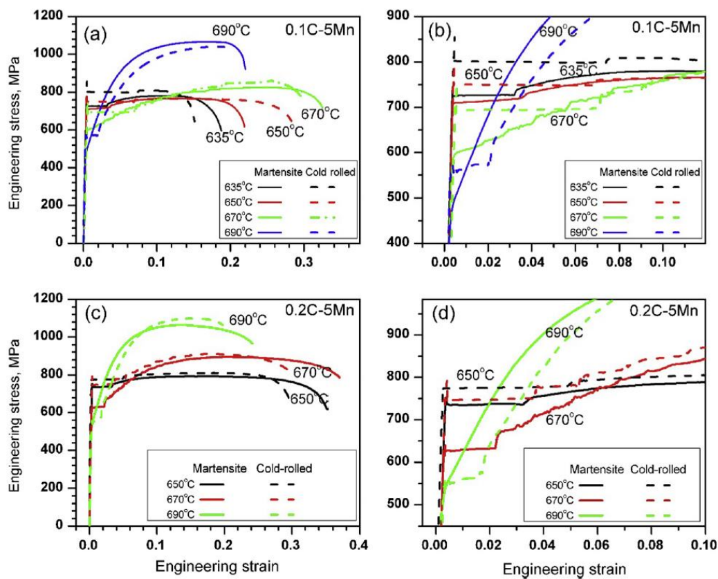
Figure 38: (a) and (c) Tensile curves of medium Mn steels with either a martensitic (continuous line) or a cold-rolled (dotted line) microstructure prior to intercritical annealing (fibrous or UFG morphologies). Two compositions are investigated (Fe/0.1C/5Mn and Fe/0.2C/5Mn). For both compositions, different intercritical annealing temperatures are investigated. (b) and (d) Magnification of the beginning of the curves to put into light the Lüders' plateau [13].
