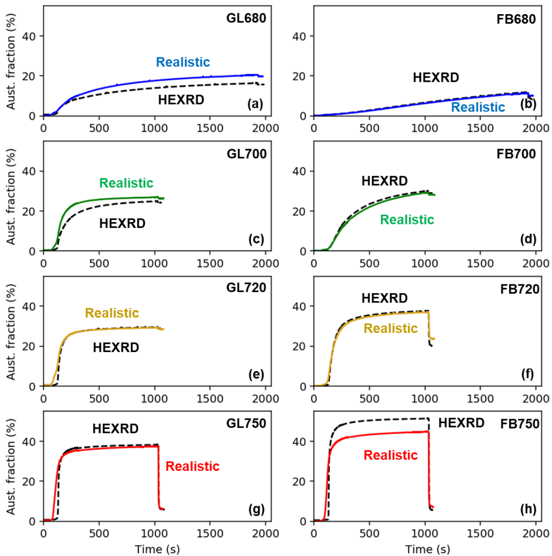
Figure 162: Austenite phase fraction as a function of time for the eight realistic experiments (coloured curves): (a) GL680, (b) FB680, (c) GL700, (d) FB700, (e) GL720, (f) FB720, (g) GL750 and (h) FB750. The kinetics obtained during “HEXRD dilatometry” experiments are reproduced from Chapter II (black dashed curve).
