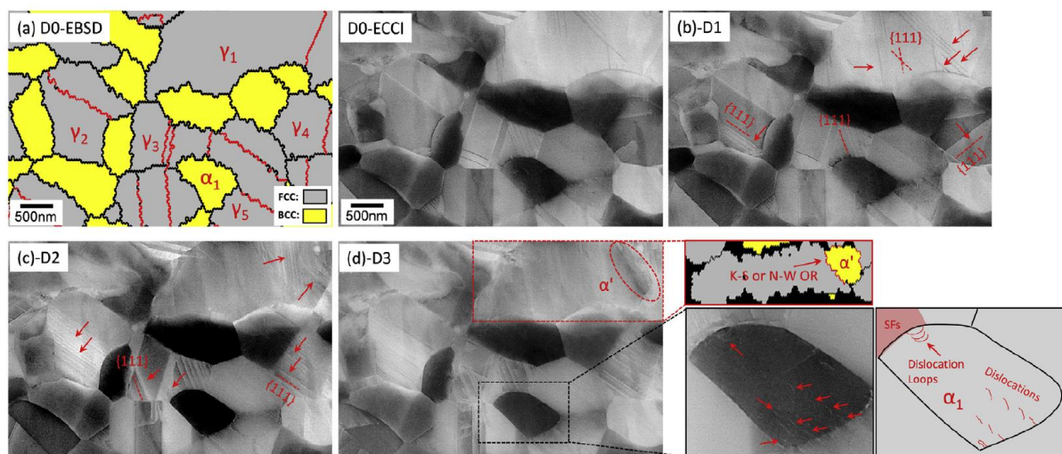
Figure 36: Microstructural evolution of a medium Mn steel during an in-situ three-point bending test. (a) EBSD map (yellow = ferrite, grey = austenite) and ECCI micrograph in the undeformed state. On the EBSD map, red lines correspond to twin boundaries. (b) (c) (d) Evolution of ECCI images of the same area with increasing strain. Red arrows indicate the formation of stacking faults and dislocations [148].
