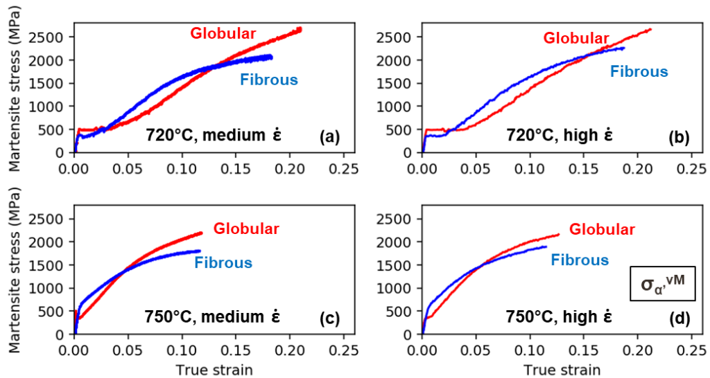
Figure 113: Martensite von Mises stress as a function of macroscopic true strain for 8 experiments: (a) T_{IA} = 720^{\circ}\text{C} , medium \dot{\epsilon} ; (b) T_{IA} = 720^{\circ}\text{C} , high \dot{\epsilon} ; (c) T_{IA} = 750^{\circ}\text{C} , medium \dot{\epsilon} ; (d) T_{IA} = 750^{\circ}\text{C} , high \dot{\epsilon} . The martensite von Mises stresses are determined using \sin^2\psi method.
