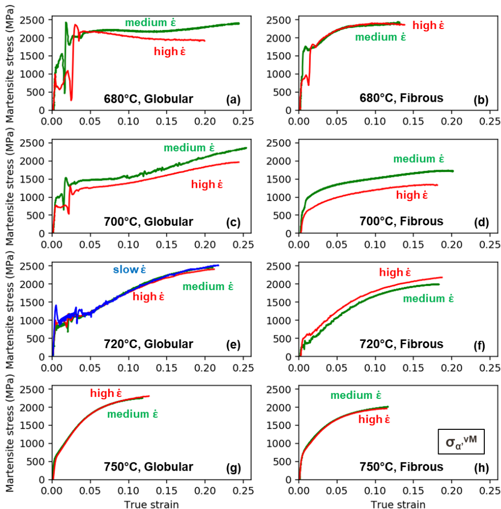
Figure 119: Martensite von Mises stress as a function of macroscopic true strain for the 17 experiments: (a) T_{IA} = 680^{\circ}\text{C} , globular; (b) T_{IA} = 680^{\circ}\text{C} , fibrous; (c) T_{IA} = 700^{\circ}\text{C} , globular; (d) T_{IA} = 700^{\circ}\text{C} , fibrous; (e) T_{IA} = 720^{\circ}\text{C} , globular; (f) T_{IA} = 720^{\circ}\text{C} , fibrous; (g) T_{IA} = 750^{\circ}\text{C} , globular; (h) T_{IA} = 750^{\circ}\text{C} , fibrous. The martensite von Mises stresses are calculated using inverse Hill's mixture rules.
