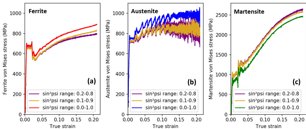
Figure 173: Effect of the \sin^2\psi range used for linear fit on the von Mises stresses in ferrite (a), austenite (b) and martensite (c) for the GL720-001 experiment. The stress in red, blue and green represents the stress obtained after linear fitting over the whole \sin^2\psi range. In gold are the curves obtained after a linear fit over 0.1-0.9 \sin^2\psi range, and in purple the ones obtained over 0.2-0.8 \sin^2\psi range.
