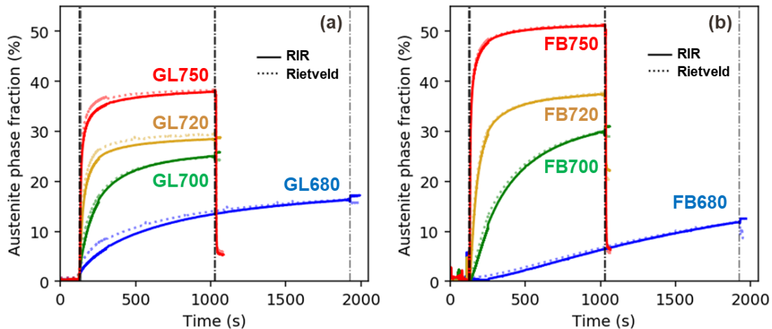
Figure 53: Comparison of the austenite phase fraction evolution determined by RIR method (solid line) and Rietveld refinement (dotted line), as a function of time for the 4 considered intercritical annealing temperatures. In (a), the initial microstructure is cold-rolled ferritic (one-step), while in (b), it is as-quenched martensitic (two-step). In (a) and (b), the first vertical line corresponds to the end of heating stage (similar values for all treatments). The second vertical line corresponds to the cooling start for 700°C, 720°C and 750°C experiments. The third line corresponds to the cooling start for 680°C experiment.
