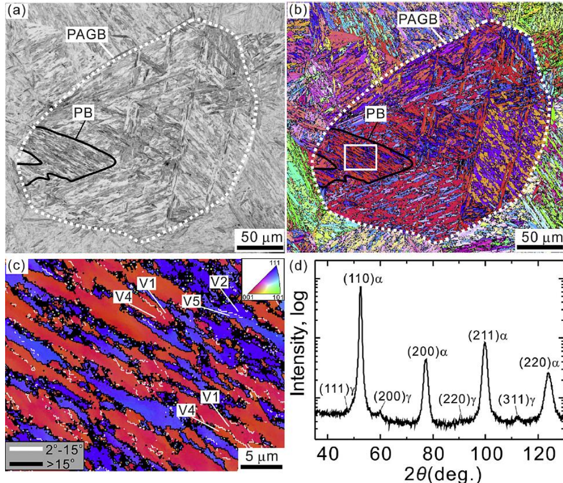
Figure 151: Martensite laths found in an as-quenched steel (Fe-2Mn-1.5Si-0.3C) observed in (a) an OM image and (b) a \alpha orientation map. PAGB corresponds to the prior austenite grain boundary, PB corresponds to the packet boundary. (c) is a zoom from the white rectangle in the (b) map, where low and high angle boundaries are indicated. (d) is the X-ray diffraction profile of the specimen [7].
