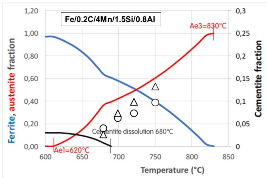
Figure 60: Fractions of ferrite (in blue), austenite (in red) and cementite (black) at the orthoequilibrium of the studied steel as a function of temperature. The experimental values obtained by HEXRD at the end of the isothermal holding have been reported (two-step: triangle, one-step: circle).
