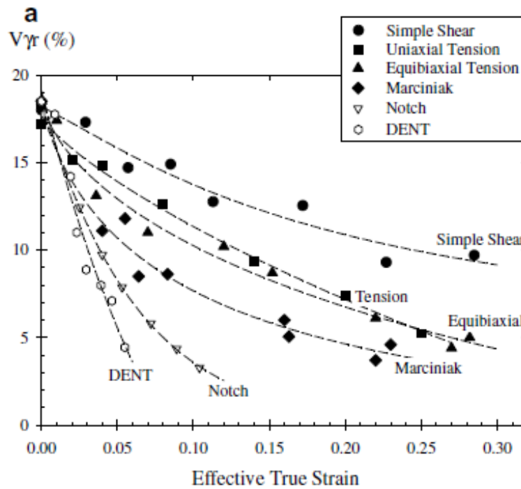
Figure 27: Evolution of the austenite volume fraction as a function of effective true strain for different stress states, in a Fe/0.3C/1.4Mn/1.4Si conventional TRIP steel [85].
