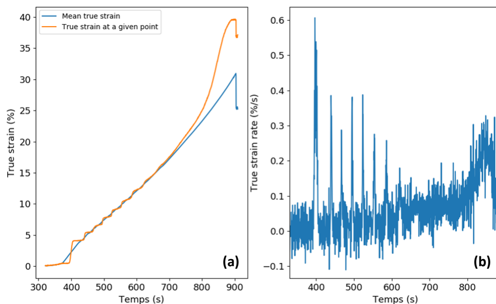
Figure 83: (a) Evolution of mean strain along the gauge length of the specimen (blue curve) and the strain at the diffracting area (orange curve) during the GL720-001 experiment. (b) Evolution of the strain rate at the diffracting area during the GL720-001 experiment.
