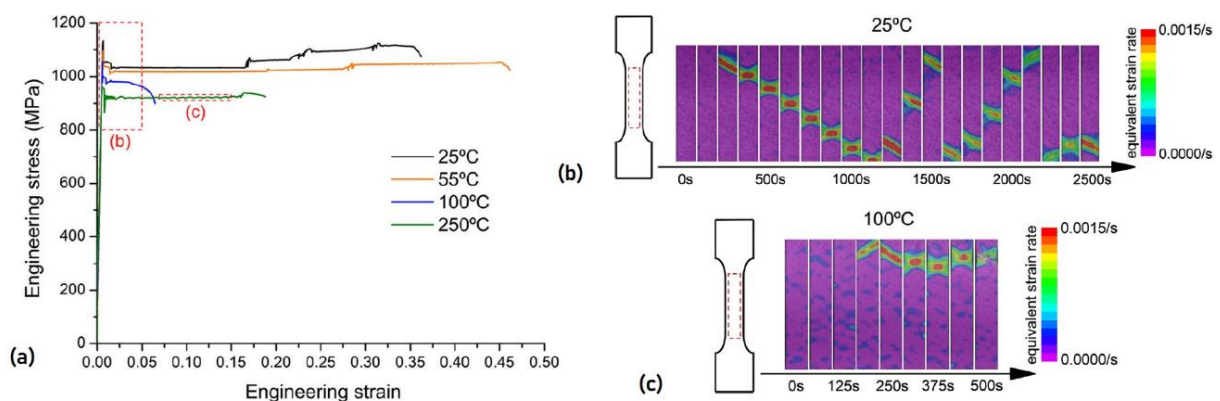
Figure 35: (a) Tensile curves of a Fe/0.14C/7.14Mn/0.23Si cold-rolled medium Mn steel, deformed at different temperatures (between 25°C and 250°C). The local strain rate maps measured in situ by DIC during tensile testing are reported for 25°C (b) and 100°C (c) for different times. Figures are extracted from [149].
