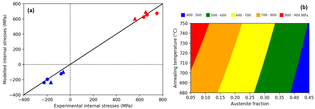
Figure 64: (a) Comparison between the experimental stress states (Table 7) in the absence of martensitic transformation and the modelled stress states (Table 8). The red symbols correspond to austenite and the blue ones to ferrite. The circles represent one-step experiments and the triangles the unique relevant two-step experiments. (b) Hydrostatic pressures predicted in austenite in an austenite fraction/annealing temperature map. The white circles correspond to the one-step experiments below 720°C.
