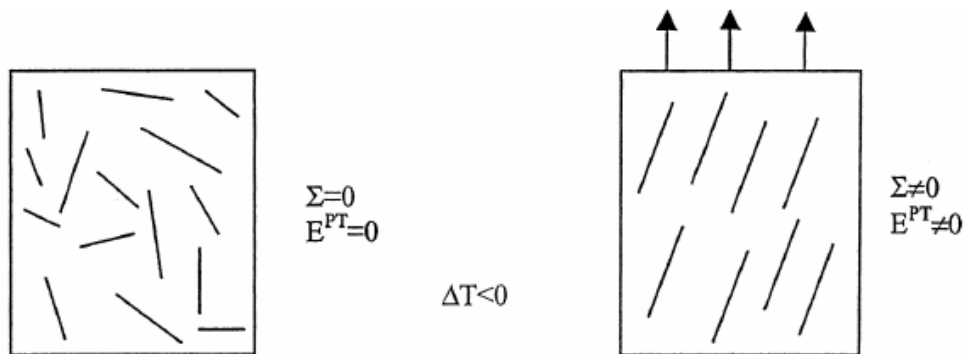
Figure 32: Representation of the Magee effect, with \Sigma the macroscopic stress and E^{PT} the plastic strain [35].
