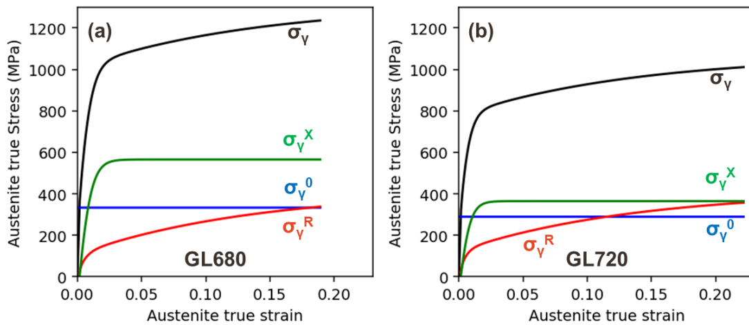
Figure 146: Decomposition of the flow stress of austenite \sigma_V (black) into different components: friction term \sigma_V^0 (blue), isotropic hardening term \sigma_V^R (red) and kinematic hardening term \sigma_V^X (green), for (a) GL680 steel and (b) GL720 steel.
