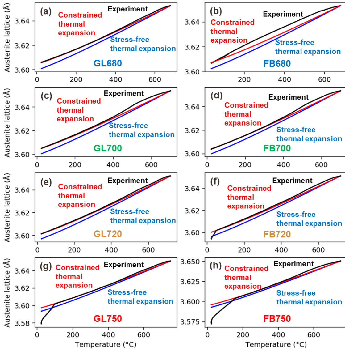
Figure 62: Austenite lattice parameters as a function of the temperature during (a), (c) (e) and (g) one-step treatments and (b), (d), (f) and (h) two-step treatments at different intercritical annealing temperatures. Experimental data in black, reproduced from Figure 57. The stress-free thermal expansions according to Equation ( II—11 ) are represented in blue and the constrained thermal expansions according to Equation ( II—13 ) in red.
