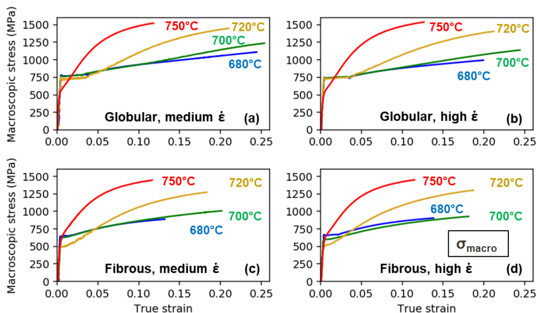
Figure 102: True tensile curves for (a) globular microstructures deformed at the medium \dot{\epsilon} , (b) globular deformed at the high \dot{\epsilon} , (c) fibrous deformed at the medium \dot{\epsilon} and (d) fibrous deformed at the high \dot{\epsilon} for the four in IA temperatures. The curves are represented up to necking.
