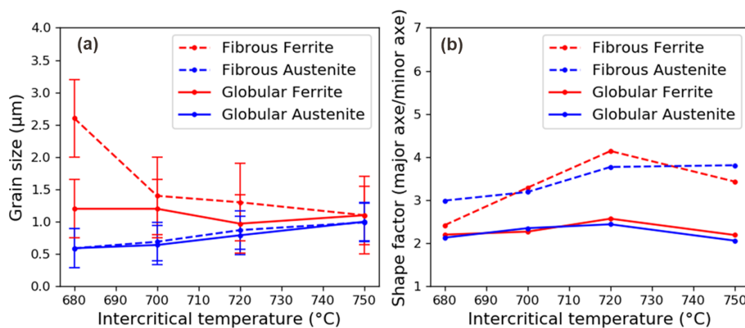
Figure 73: Average grain sizes (a) and shape factors (b) of the two phases as a function of the intercritical annealing temperature for both microstructure morphologies. The bars on (a) are representative of the standard deviation of grain size distributions. They are not represented in (b) for clarity purpose.
