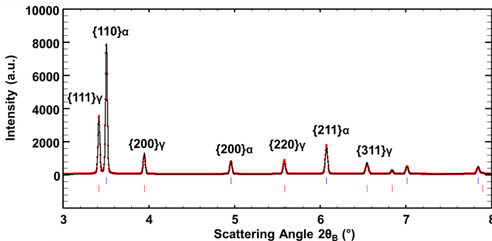
Figure 50: Example of a Rietveld refinement. In red: experimental points of the diffractogram. In black: the theoretical line profile. The plane families are given above the corresponding peaks.
