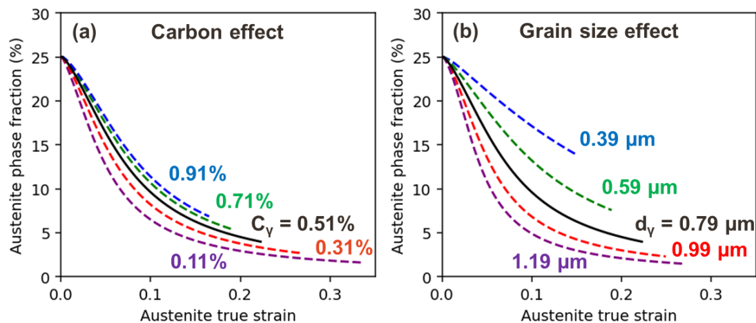
Figure 143: (a) Comparison of the evolution of austenite phase fractions in GL720 steel when the carbon content of austenite C_v is modified. (b) Comparison of the evolution of austenite phase fractions in GL720 steel when the grain size of austenite d_v is modified. For (a) and (b), the black solid curve corresponds to the reference simulation, when C_v and d_v are at their real values.
