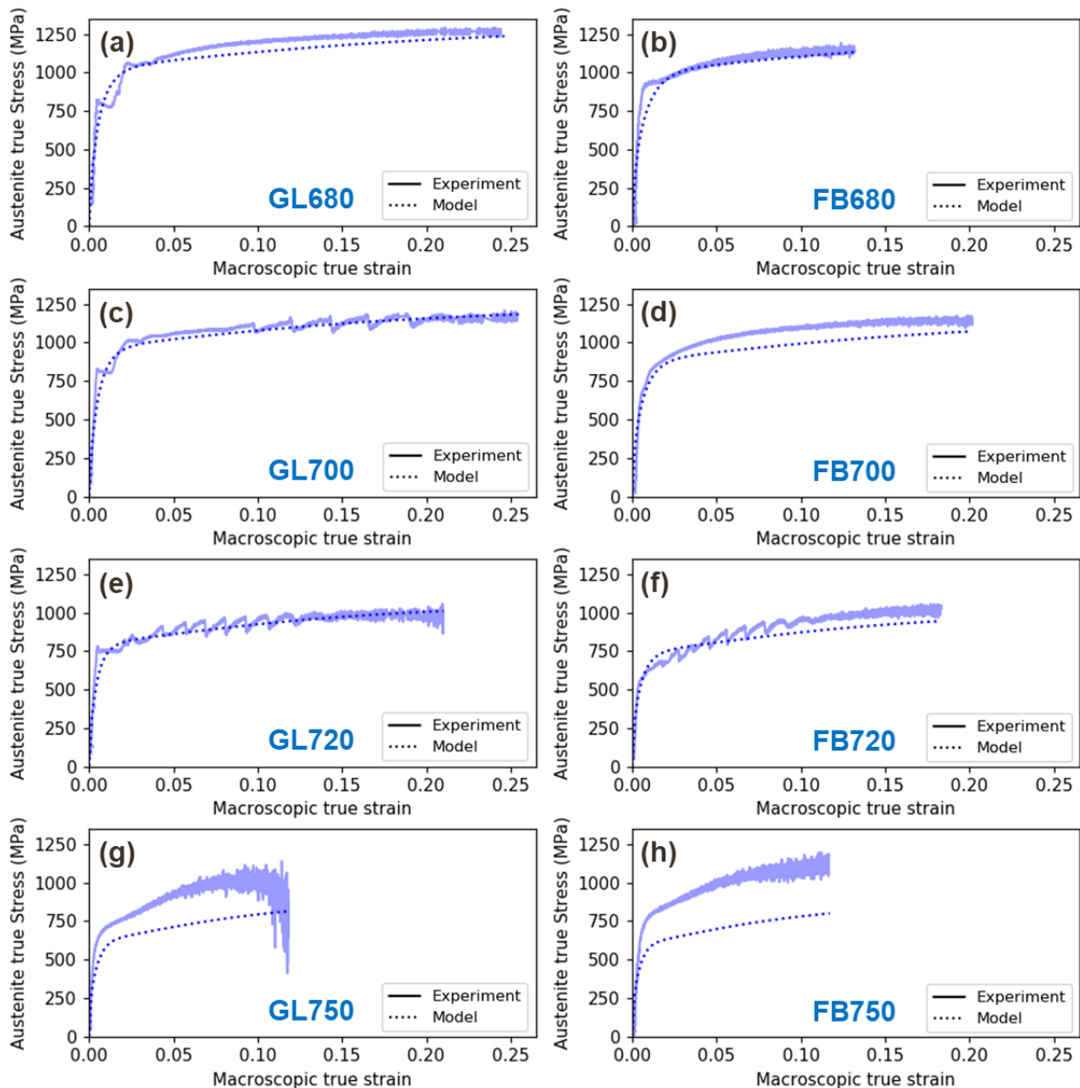
Figure 129: Comparison between the simulated flow stress (dotted line) and the experimental von Mises stress (solid line) in austenite for (a) GL680, (b) FB680, (c) GL700, (d) FB700, (e) GL720, (f) FB720, (g) GL750, (h) FB750 steels respectively. The stresses in austenite are displayed as a function of \epsilon_{\text{macro}} .
