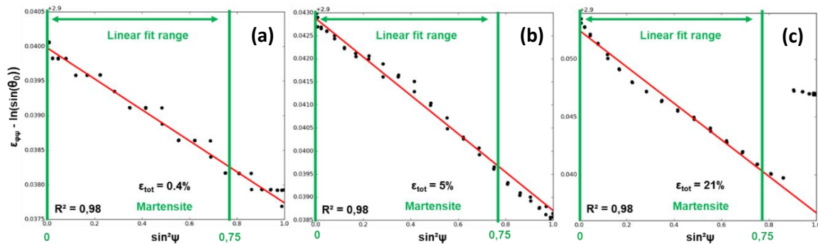
Figure 87: Evolution of martensite \sin^2\psi ellipses (black dots) as a function of strain during GL720-001 experiment. At \epsilon=0.4\% (a), the steel is still in elastic regime. At \epsilon=5\% (b), the Lüders band has come across all the specimen length. At \epsilon=21\% (c), necking starts. The linear regression (red line) was conducted over a \sin^2\psi range of [0; 0.75] , indicated by green vertical line. For each regression, the R^2 values is systematically higher than 0.98.
