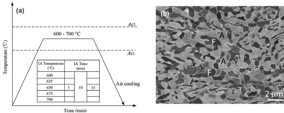
Figure 9: (a) Typical intercritical annealing to produce UFG medium Mn steels and (b) globular dual phase UFG microstructure observed by SEM resulting from an intercritical annealing at 700°C of a cold rolled Fe/0.6C/6.6Mn/3Al steel. A stands for Austenite and F for Ferrite, taken from [4], [5].
