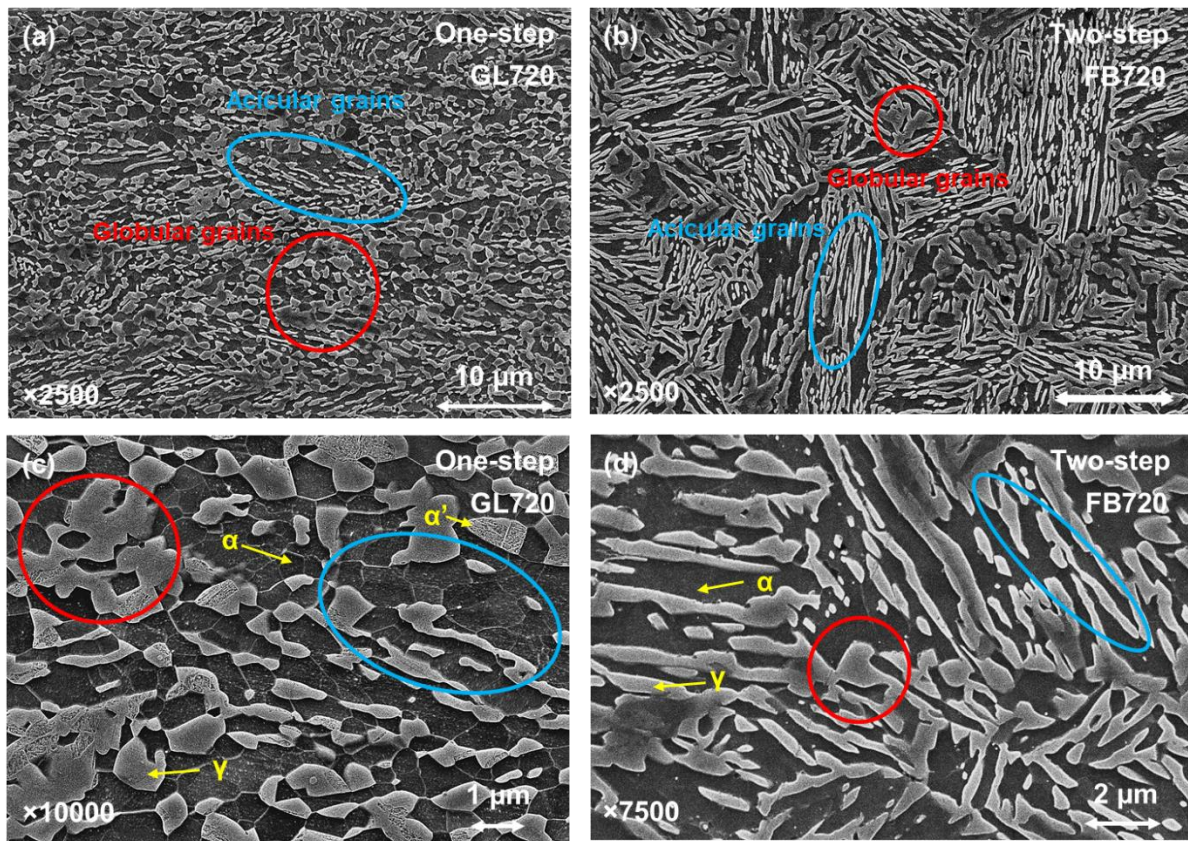
Figure 70: SEM micrographs of globular and fibrous microstructures annealed at 720°C. (a) GL720 magnified at \times 2500 . (b) FB720 magnified at \times 2500 . (c) GL720 magnified at \times 10000 . (d) FB720 magnified at \times 7500 . Ferrite appears in dark grey, austenite in light grey, cementite in white particles.
