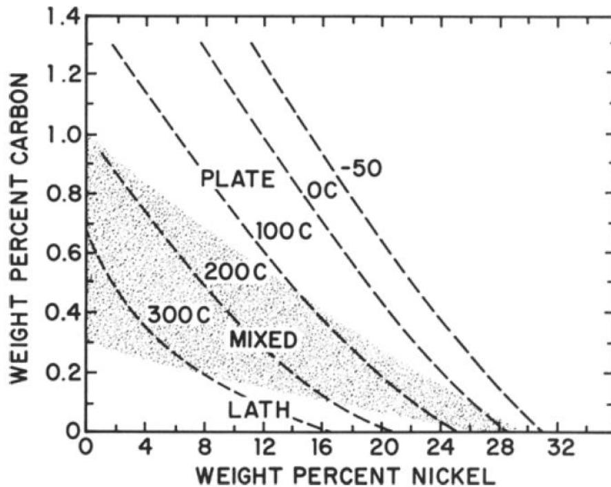
Figure 152: The morphology of martensite as a function of the composition in Ni and C of the former austenite. The dashed-line correspond to isopleths of M_s temperature [228].
