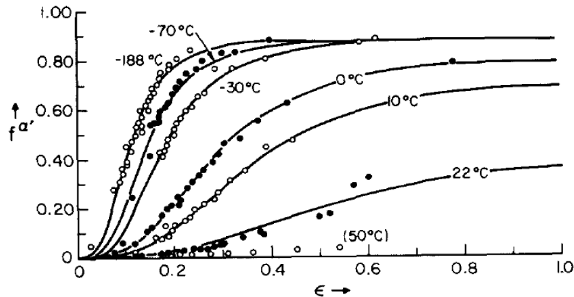
Figure 29: Comparison between the experiments conducted by Angel et al. [101] on a 304 stainless steel (dots) and the simulations using Olson and Cohen equations (reproduced from [11]).
