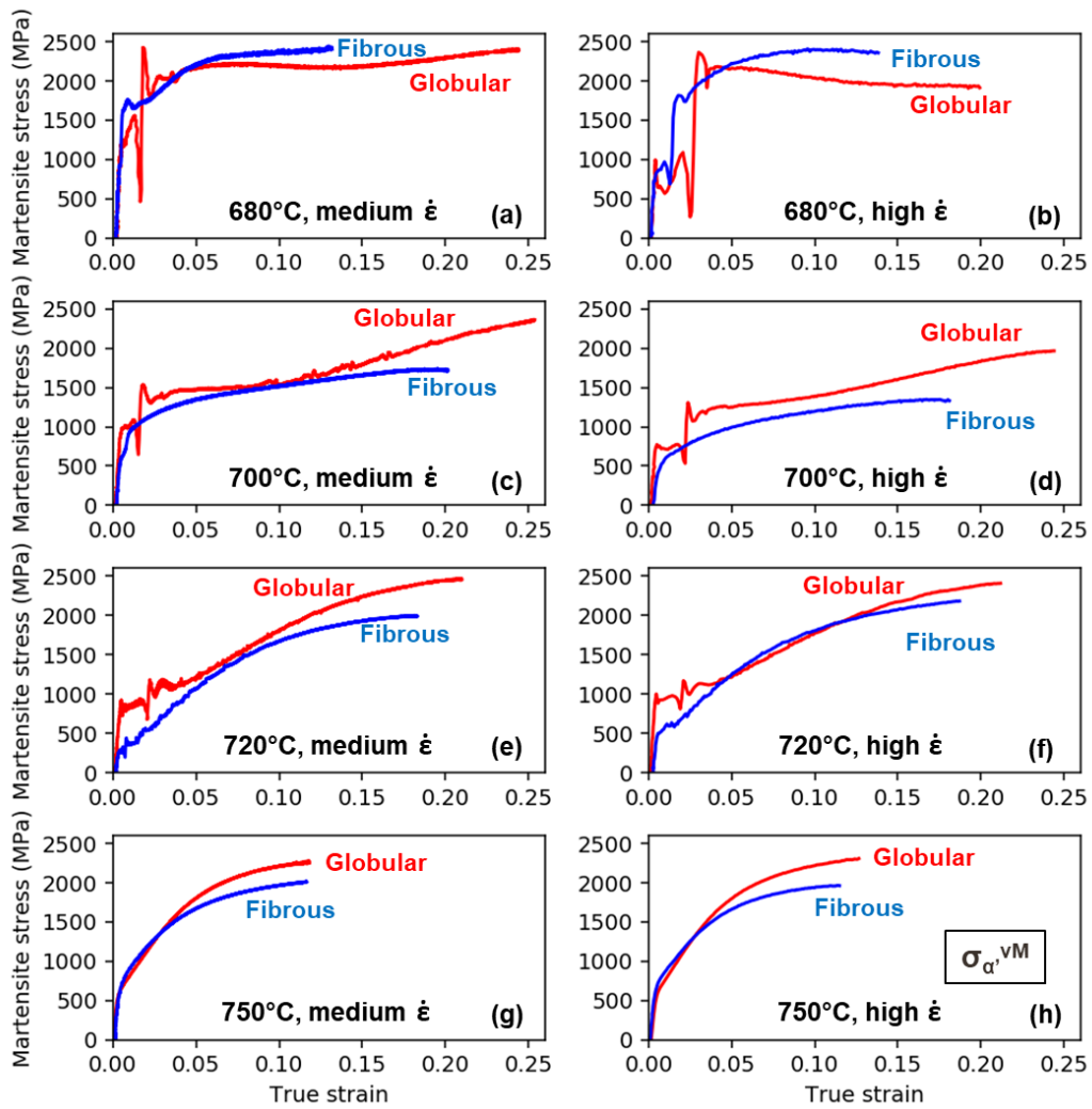
Figure 112: Martensite von Mises stress as a function of macroscopic true strain for the 16 experiments at the two higher strain rates: (a) T_{IA} = 680^{\circ}\text{C} , medium \dot{\epsilon} ; (b) T_{IA} = 680^{\circ}\text{C} , high \dot{\epsilon} ; (c) T_{IA} = 700^{\circ}\text{C} , medium \dot{\epsilon} ; (d) T_{IA} = 700^{\circ}\text{C} , high \dot{\epsilon} ; (e) T_{IA} = 720^{\circ}\text{C} , medium \dot{\epsilon} ; (f) T_{IA} = 720^{\circ}\text{C} , high \dot{\epsilon} ; (g) T_{IA} = 750^{\circ}\text{C} , medium \dot{\epsilon} ; (h) T_{IA} = 750^{\circ}\text{C} , high \dot{\epsilon} . The von Mises stresses are calculated with Hill's mixture rules.
