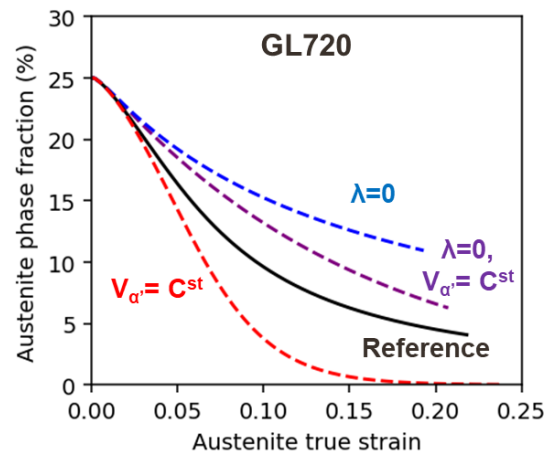
Figure 144: Evolution of the SIMT kinetics for the GL720 steel when the model is modified. The black solid curve is the reference simulation. The blue curve ( \lambda = 0 ) corresponds to the absence of autocatalytic transformation. The red curve ( V_\alpha = C^{st} ) corresponds to a simulation where the volume of martensite remains constant across the simulation, calculated as V_\alpha = S_\alpha d_v^0 . The purple curve corresponds to the superposition of the two precedent modifications to SIMT constitutive laws.
