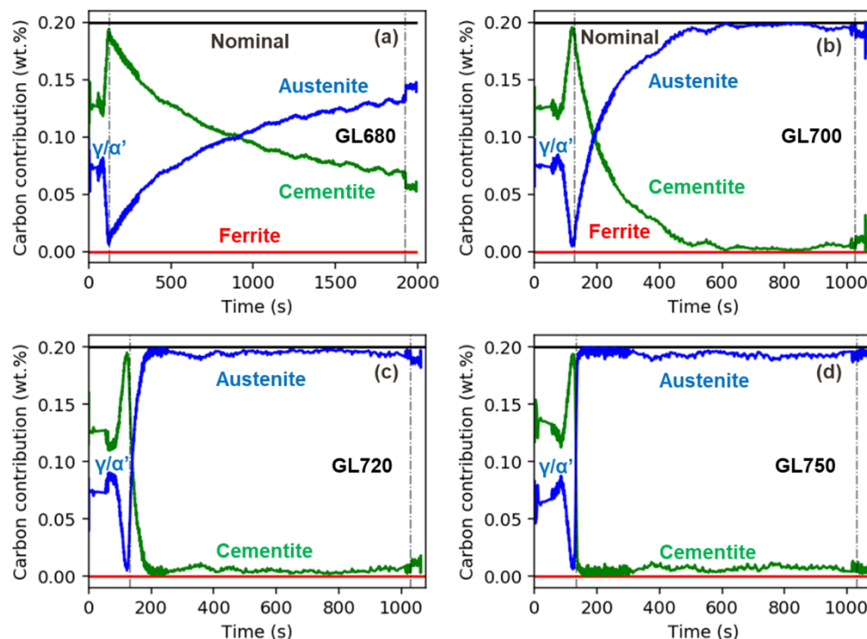
Figure 155: Repartition of the carbon between each phase of the globular steels: ferrite (red), austenite (blue), cementite (green). The nominal carbon content is indicated by the black line. (a) For GL680, (b) for GL700, (c) for GL720 and (d) for GL750 experiments. The first vertical line corresponds to heating end. The second vertical line corresponds to cooling start. A moving average filter was used to smooth the curves (10 closest neighbours).
