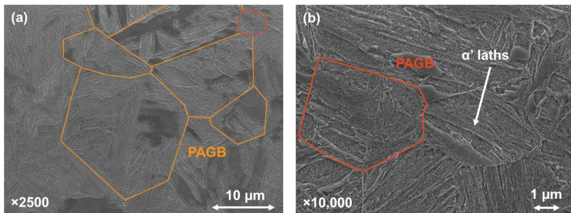
Figure 45: SEM micrographs of the martensitic steel (a) at a magnification of \times 2500 and (b) at a magnification of \times 10,000 . The rolling direction is horizontal. The microstructure consists of martensite laths. PAGB correspond to the prior austenite grain boundaries (in orange and red). The red contoured island is the same between (a) and (b).
