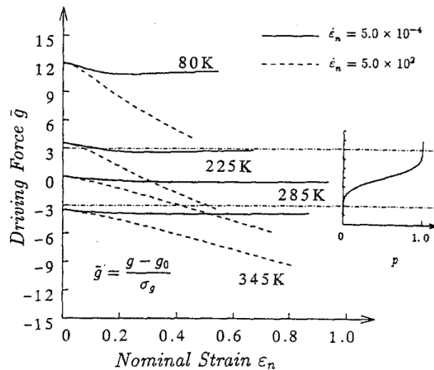
Figure 154: Normalized driving force \bar{g} for the martensitic transformation as a function of the strain. Its evolution is given for 4 temperatures and 2 strain rates. In solid line are the evolution of \Delta G^{V \rightarrow \alpha} at low strain rate ( 5 \times 10^{-4} \text{ s}^{-1} ). In dashed line are the evolution of \Delta G^{V \rightarrow \alpha} at high strain rate ( 5 \times 10^2 \text{ s}^{-1} ) [120].
