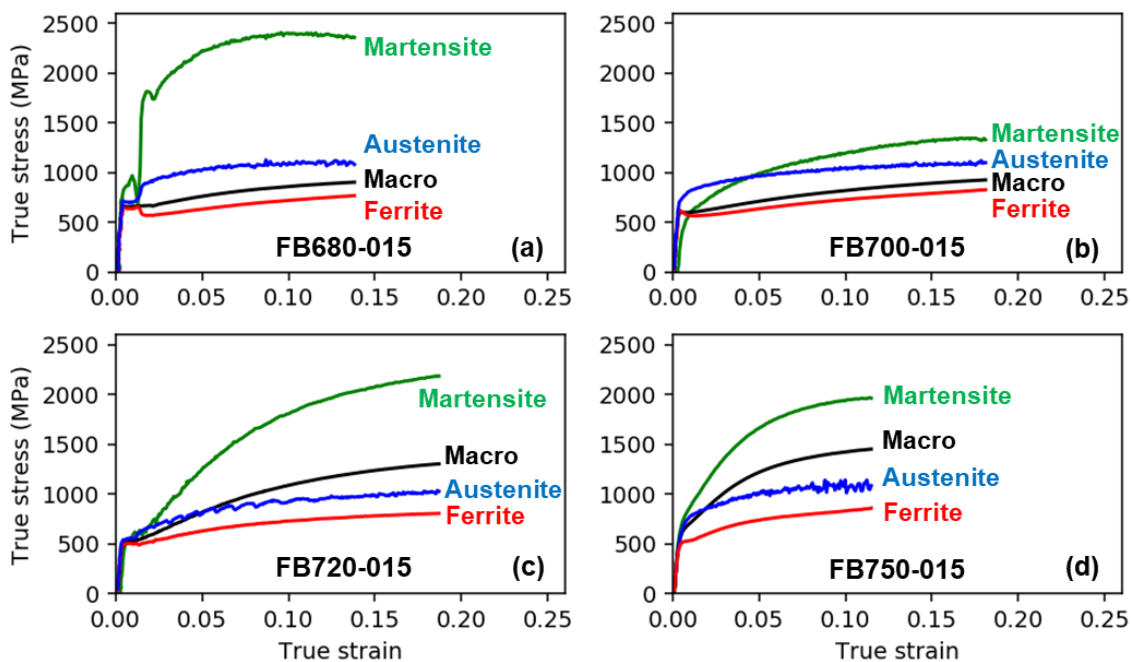
Figure 99: Comparison between the macroscopic stress \sigma_{tot} (black), the von Mises stresses in ferrite \sigma_{\alpha}^{vM} (red) and austenite \sigma_{\gamma}^{vM} (blue) determined by \sin^2\psi method and the von Mises stress in martensite \sigma_{\alpha'}^{vM} (green) calculated by the mixture rule for the four samples with the fibrous microstructure strained at the high rate. (a) FB680-015. (b) FB700-015. (c) FB720-015. (d) FB750-015.
