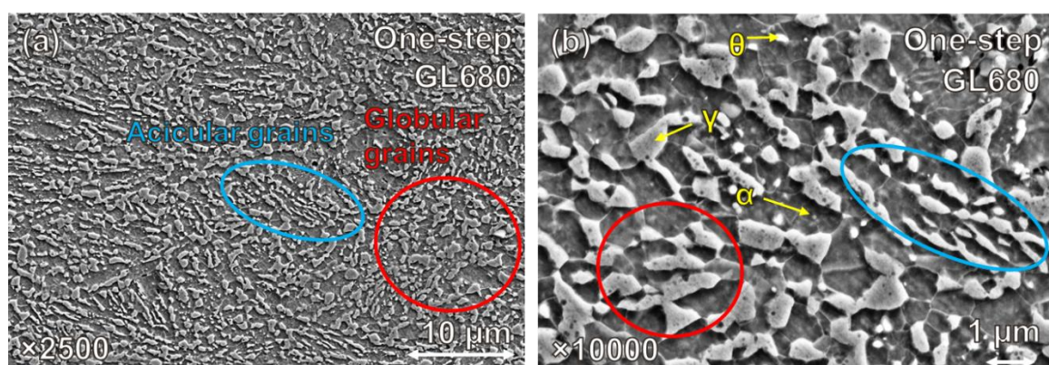
Figure 157: SEM micrographs of globular microstructures produced at 680°C in HEXRD dilatometry (microstructure formation described in Chapter II). (a) GL680 magnified at \times 2500 . (b) GL680 magnified at \times 10000 . Ferrite appears in dark grey, austenite in light grey, cementite in white particles.
