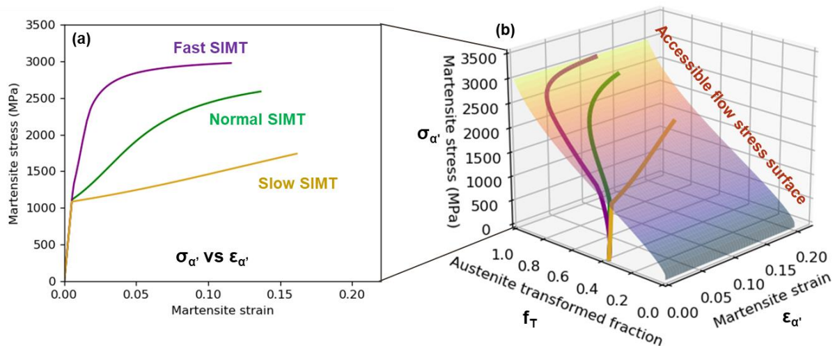
Figure 147: (a) Model \sigma_{\alpha'} vs \varepsilon_{\alpha'} curves for the GL720 microstructure for the three tested SIMT kinetics (Slow: yellow; Correct: green; Fast: purple). (b) 3D surface of accessible flow stress for martensite \sigma_{\alpha'} as a function of its strain \varepsilon_{\alpha'} and the fraction of transformed austenite f_{\tau} . The 3 curves from (a) have been plotted in 3D space by adding their dependence on f_{\tau} . After elastic domain, the curves are superimposed to the master surface.
