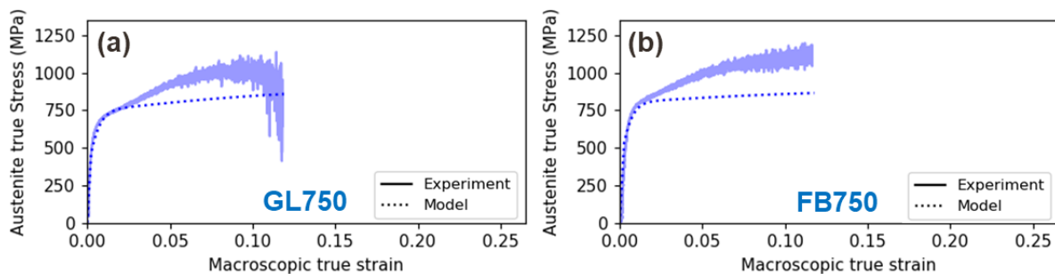
Figure 130: Comparison between the simulated flow stress (dotted line) and the experimental von Mises stress (solid line) in austenite for (a) GL750 and (b) FB750 steels. The difference with Figure 129 (g) and (h) is that the initial density dislocation \rho_v^0 is increased to 1 \times 10^{14} \text{ m}^{-2} for GL750 and 2 \times 10^{14} \text{ m}^{-2} for FB750. The stresses in austenite are displayed as a function of \epsilon_{\text{macro}} .
