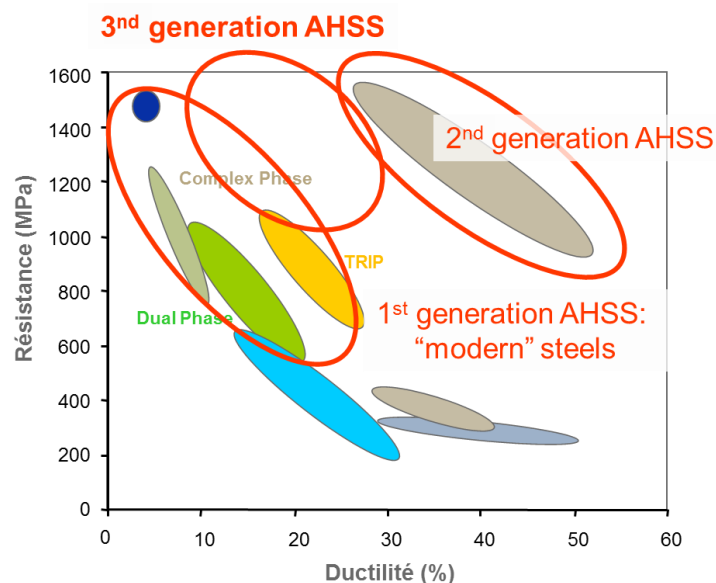
Figure 7: Comparison of the strength and ductility of different generations of AHSS [28]. The domain for 3 rd generation AHSS is still a target as few products have really been put into production so far.
