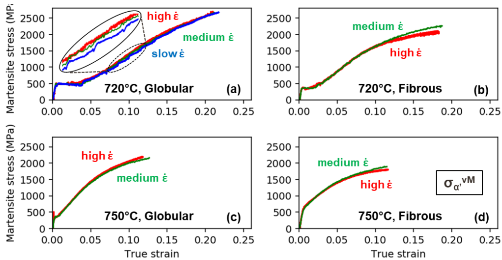
Figure 120: Martensite von Mises stress as a function of macroscopic true strain at different strain rates: (a) T_{IA} = 720^{\circ}\text{C} , globular; (b) T_{IA} = 720^{\circ}\text{C} , fibrous; (c) T_{IA} = 750^{\circ}\text{C} , globular; (d) T_{IA} = 750^{\circ}\text{C} , fibrous. The martensite von Mises stresses are calculated using \sin^2\psi method.
