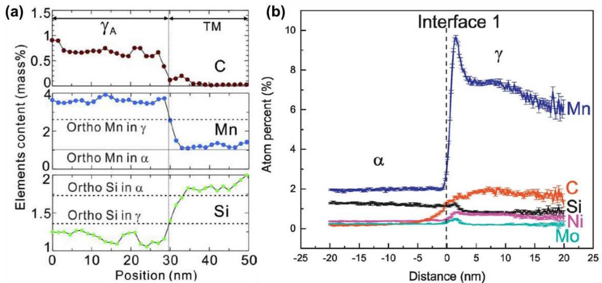
Figure 20: (a) Profiles measured by APT of C, Mn and Si across acicular austenite \gamma_A and thermal martensite TM interface [65]. (b) Profiles measured by APT of C, Mn, Si, Ni and Mo across acicular austenite \gamma and ferrite \alpha interface [72]. From a thermal processing viewpoint, only one IA has been conducted in (a), while there have been two consecutive IA in (b).
