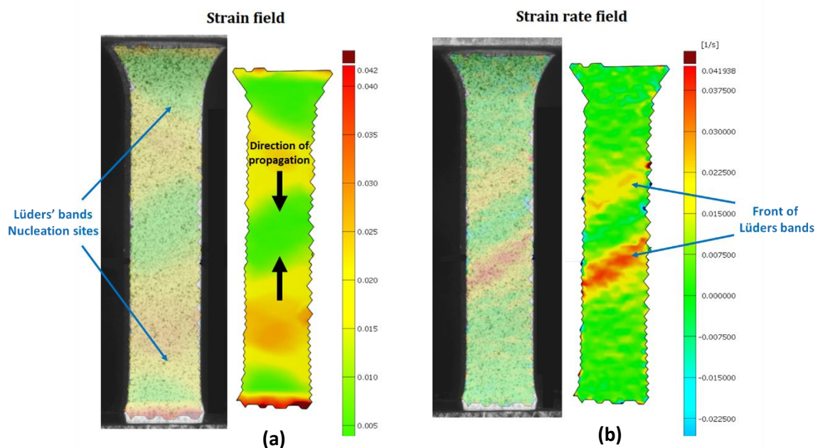
Figure 82: Strain map (a) and strain rate map (b) determined with ARAMIS system at the middle of the Lüders plateau during FB680-015 experiment (colour maps superimposed on the sample in its deformed state). The higher values of strain/strain rate appear in red. In this experiment, two Lüders bands have nucleated at each end of the tensile specimen.
