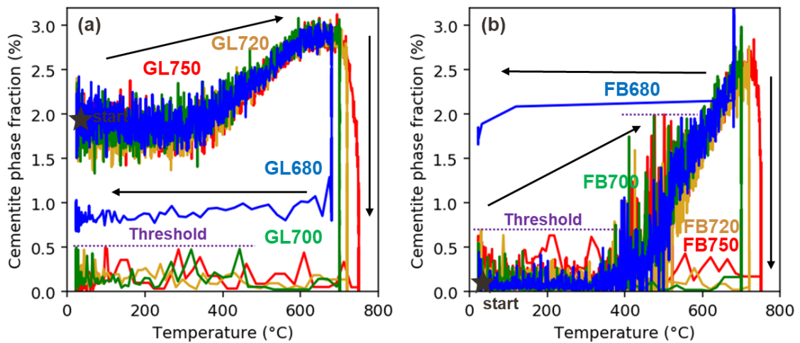
Figure 59: Cementite phase fraction as a function of temperature for the 4 considered intercritical annealing temperatures. (a) one-step experiments; (b) two-step experiments. The initial state prior to intercritical annealing is indicated by a black star. Arrows indicate the time evolution of the thermal treatment.
