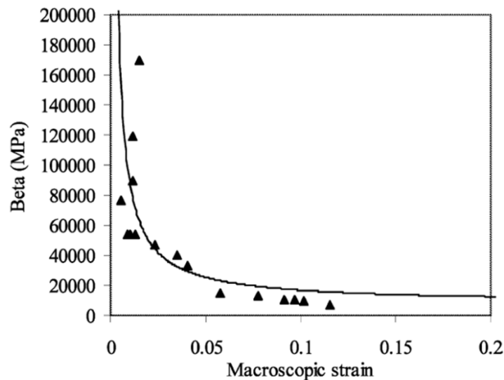
Figure 30: Comparison between the experimental (dots) and theoretical (line) stress-strain partitioning parameter \beta [8].
