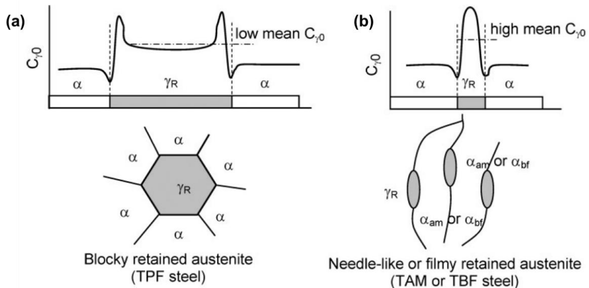
Figure 19: Illustration of the carbon concentration distribution expected in retained austenite of three kinds of TRIP aided steels. Carbon profile across retained austenite \gamma_R of TRIP steel with polygonal ferrite (TPF) is represented in (a). The one of TRIP steels with either annealed martensite (TAM) or bainitic ferrite (TBF) matrix is represented in (b) [67].
