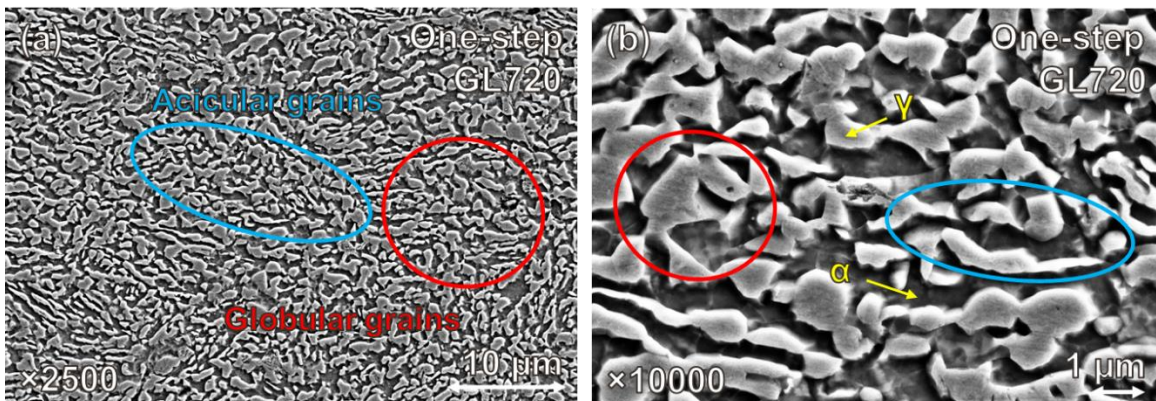
Figure 159: SEM micrographs of globular microstructures produced at 720°C in HEXRD dilatometry (microstructure formation described in Chapter II). (a) GL720 magnified at \times 2500 . (b) GL720 magnified at \times 10000 . Ferrite appears in dark grey, austenite in light grey, cementite in white particles.
