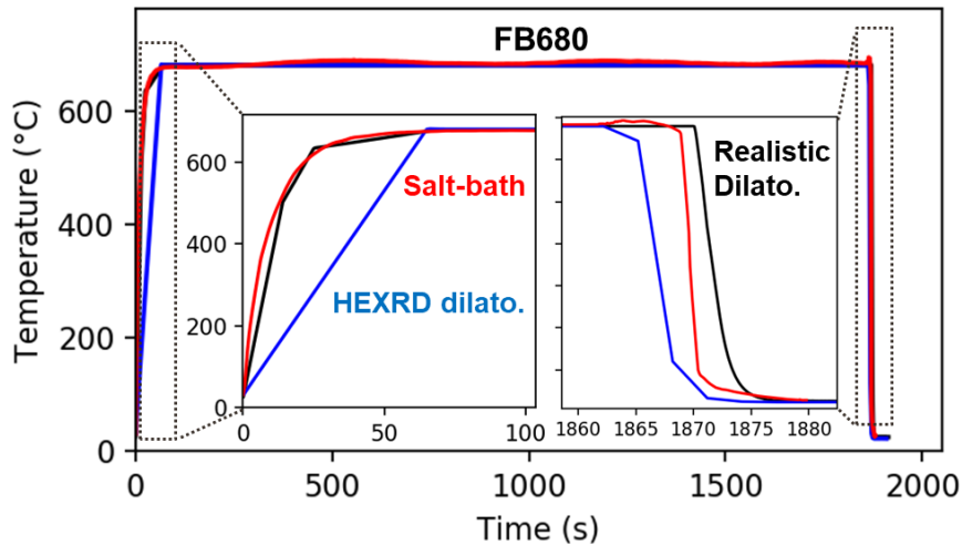
Figure 65: Comparison between the different methods used in the PhD project to produce intercritical annealed medium Mn steels. In red: treatment in salt-bath (used to produce tensile samples – cf. Chap. III). In blue: HEXRD experiments (analysed from section II.1 to II.4). In black: dilatometry treatment trying to reproduce more closely the treatment in salt-bath. The given examples are FB680 thermal treatments. Magnifications of the heating and cooling steps are also given.
