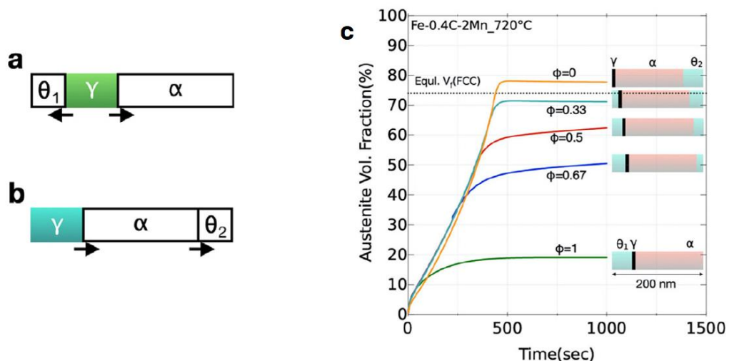
Figure 13: (a) - (b) Schematic representations of the two encountered nucleation mechanisms for austenite in cold-rolled ferritic steels during intercritical annealing. The arrows indicate the directions of interface displacements. (c) Effect of the proportion \phi of \theta_1 cementite initially presents in the microstructure on the simulation of austenite formation kinetics [57].
