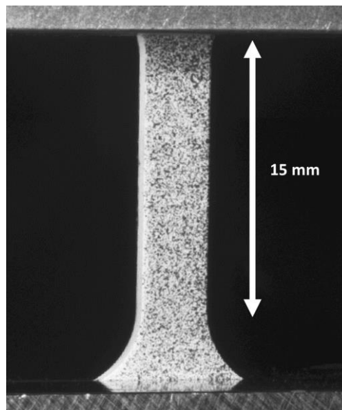
Figure 80: Speckle pattern harboured by the tensile specimen placed on a tensile tester, during the GL720-0001 experiment, just before loading.
