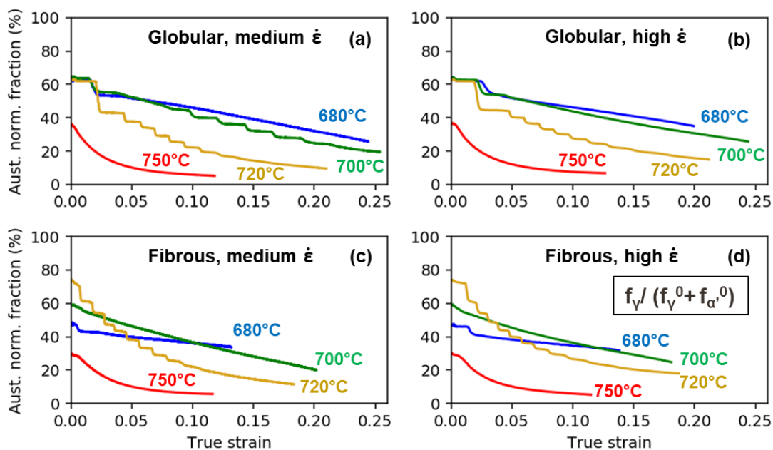
Figure 105: Austenite normalized phase fractions as a function of the macroscopic true strain for the 16 experiments at the two higher strain rates: (a) globular, medium \dot{\epsilon} ; (b) globular, high \dot{\epsilon} ; (c) fibrous, medium \dot{\epsilon} ; (d) fibrous, high \dot{\epsilon} .
