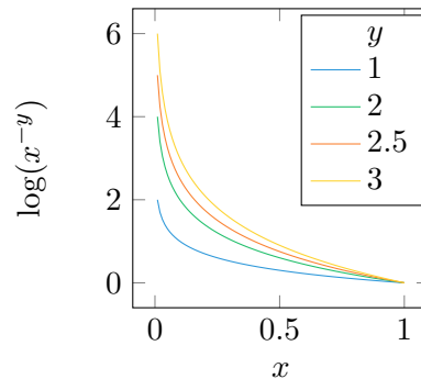
Figure 2.2: Power law distribution.
