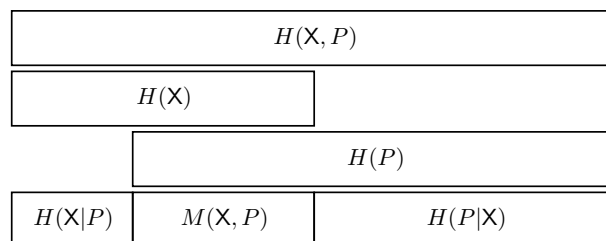
Figure 2.3: How the mutual information relate to the join entropy, individual entropies, and conditional entropies. The figure is adapted from [Mac03].
