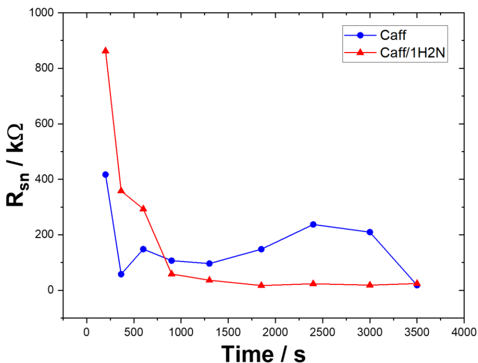
Figure 5.7: The low frequency noise impedance calculated for Scheme 5.1 electrochemical cell 12 in the absence (●) and in the presence (▲) of 1H2N. Caffeine is present for both experiments.
