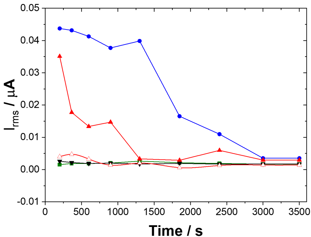
Figure 5.6: Root mean square of PSD_1 . Experimental conditions were: absence of Caff and 1H2N (▼); absence of Caff and presence of 1H2N (■); presence of Caff and absence of 1H2N (●); presence of Caff and 1H2N (▲ and △). Full symbols represent data collected with positive interfacial potential. Interface potential was negative for hollow symbols.
