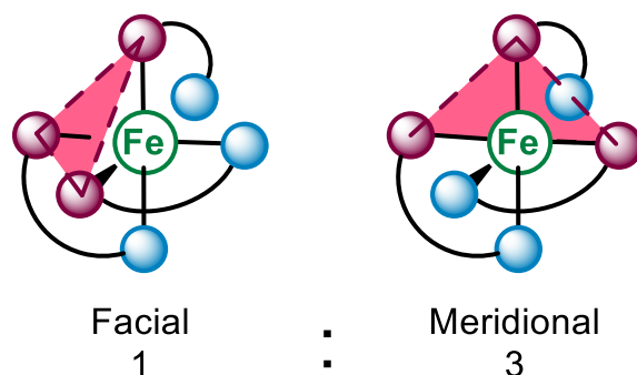
Figure 37. Representation of fac - FeL_3 and mer - FeL_3 complexes.
