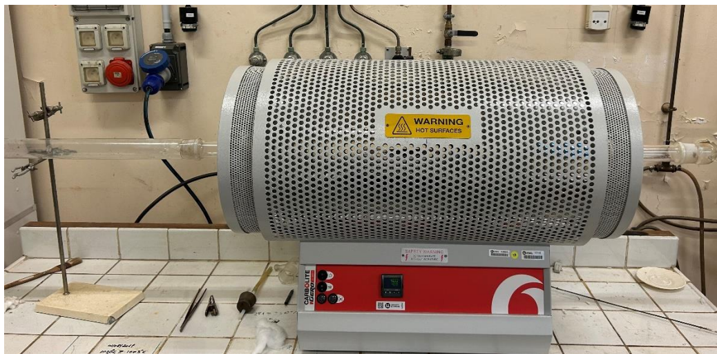
Figure 3.3: Experimental set-up for thermal treatment of samples.
