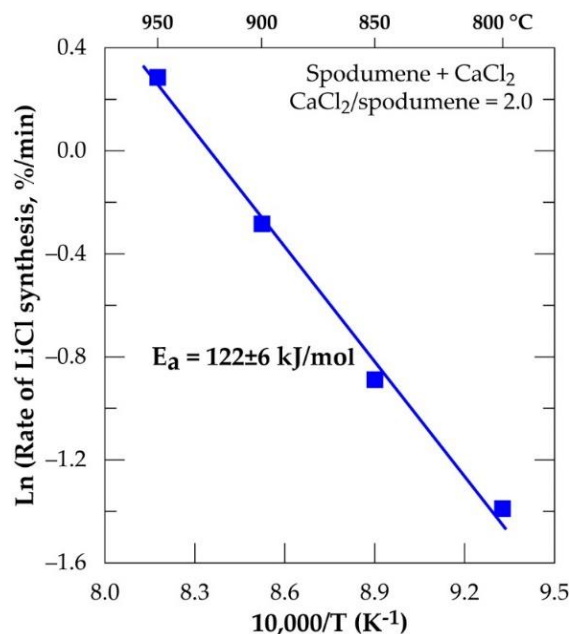
Figure 4.6: Arrhenius diagram for lithium recovery during chlorination of spodumene concentrate between 800 and 950°C, residence time = 60 minutes, CaCl 2 /spodumene = 2.0.
