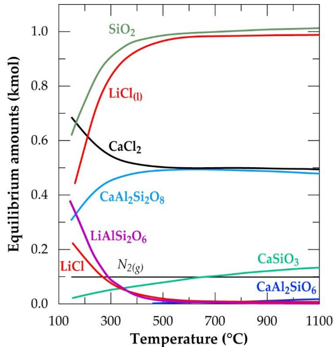
Figure 4.3: Equilibrium amounts as a function of temperature for chlorination of \alpha -spodumene using CaCl 2 (data from HSC Chemistry®5.1).
