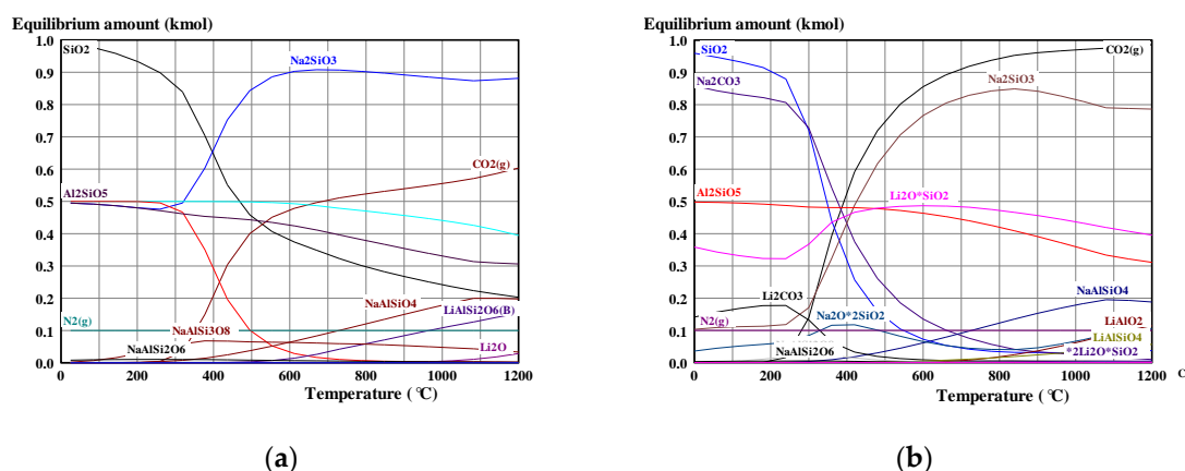
Figure 6. Equilibrium amounts versus temperature for carbonizing roasting of spodumene using \text{Na}_2\text{CO}_3 by considering reactions reported in (a) Equation (12) and in (b) Equation (13), leading to the formation of \text{Li}_2\text{O} and \text{Li}_2\text{CO}_3 , respectively (data from HSC Chemistry 5.1 software).
