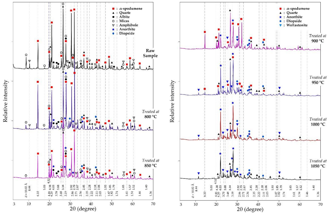
Figure 4.9: XRD pattern of evolving phases as a function of temperature at 60 minutes treatment and MR = 2.0.
