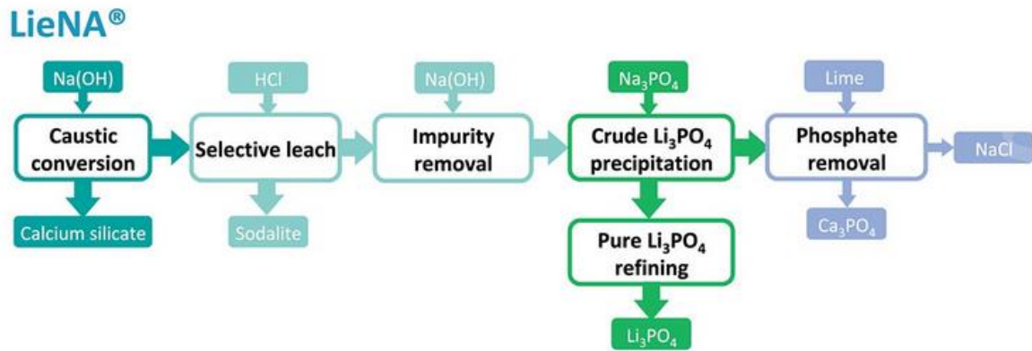
Figure 1.25: Flow diagram of LieNA® process to recover lithium phosphate [103].
