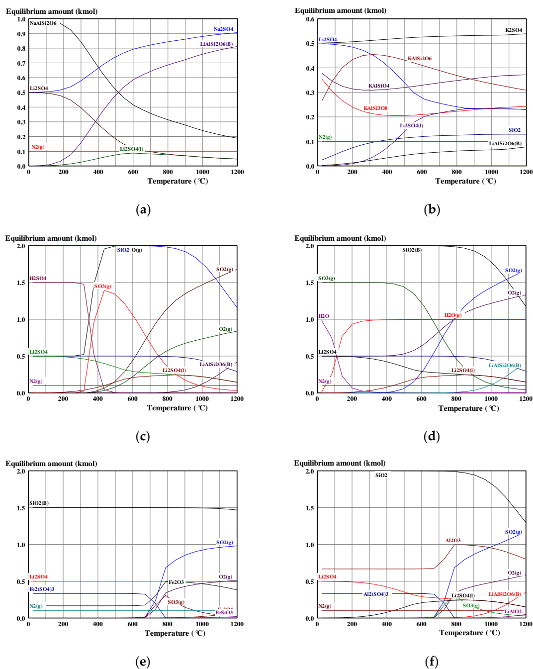
Figure 3. Equilibrium amounts versus temperature for sulfate roasting of spodumene using (a) \text{Na}_2\text{SO}_4 , (b) \text{K}_2\text{SO}_4 , (c) \text{H}_2\text{SO}_4 , (d) \text{SO}_3(\text{g}) , (e) \text{Fe}_2(\text{SO}_4)_3 and (f) \text{Al}_2(\text{SO}_4)_3 (data from HSC Chemistry 5.1 software).
