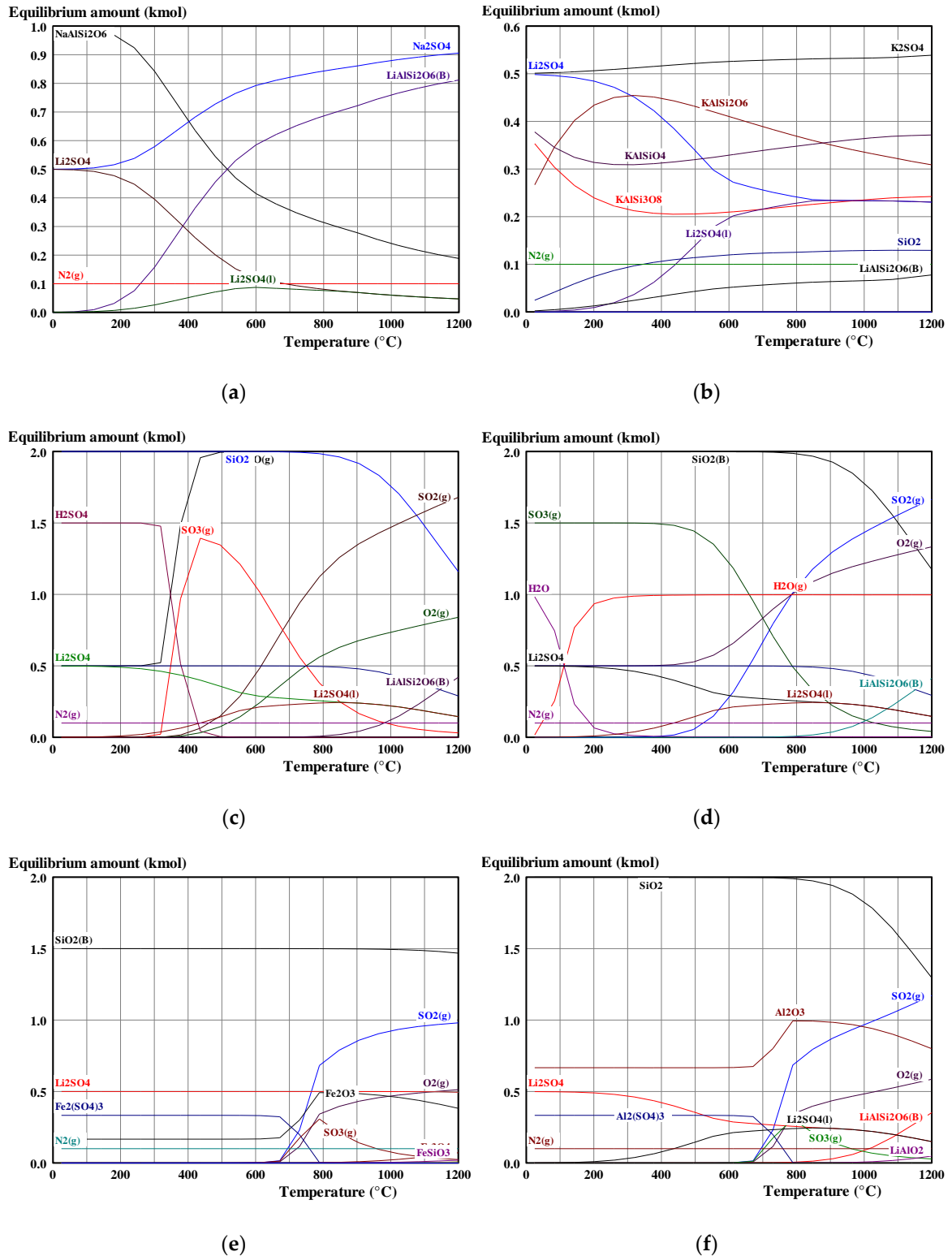
Figure 1.30: Equilibrium amounts versus temperature for sulphate roasting of spodumene using (a) \text{Na}_2\text{SO}_4 , (b) \text{K}_2\text{SO}_4 , (c) \text{H}_2\text{SO}_4 , (d) \text{SO}_3(\text{g}) , (e) \text{Fe}_2(\text{SO}_4)_3 and (f) \text{Al}_2(\text{SO}_4)_3 (data from HSC Chemistry 5.1 software).
