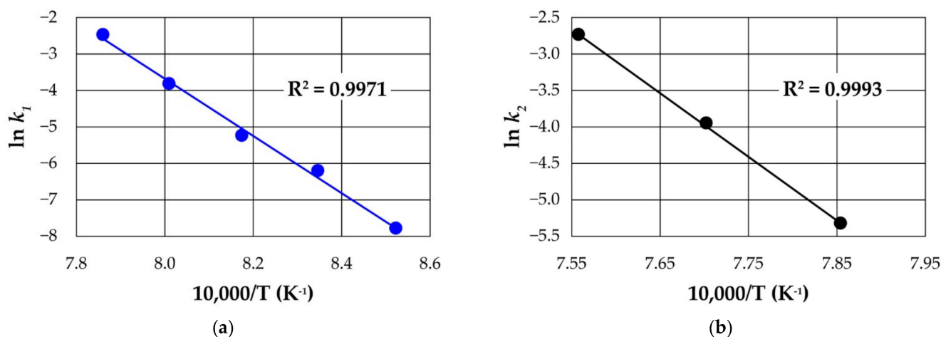
Figure 12. (a) \ln k_1 against temperature (b) \ln k_2 against temperature employing first-order kinetic model rate constants of decay plotted in Arrhenius form.
