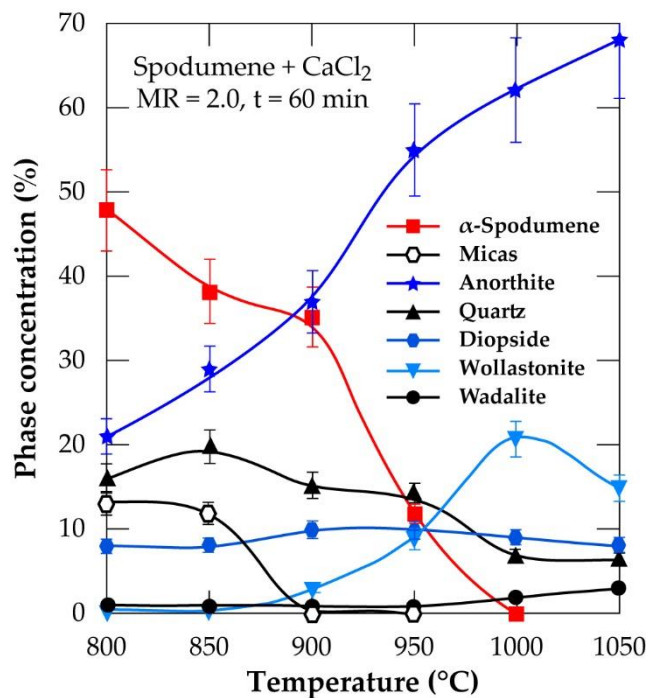
Figure 4.10: XRD semi-quantification of phases at varying temperatures for 60 minutes treatment and MR = 2.0.
