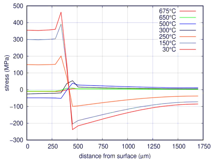
Figure IV.45: Nitrided gradient sample, in situ HEXRD experiment. Profiles of radial stress along the cylinder axis, according to the simulation and at different temperatures.
