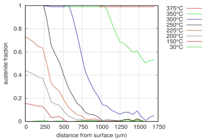
Figure IV.52: Carbonitrided sample, quench into oil. Profiles of austenite fraction, according to the simulation and at different temperatures.
