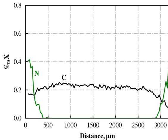
Figure III.12: Carbon and nitrogen composition profile in the nitrated gradient sample (oil quench).
