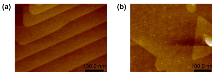
Figure 58. AFM scanning images of \text{Bi}_2\text{Te}_3 and \text{Fe}_3\text{GeTe}_2/\text{Bi}_2\text{Te}_3 heterostructures
