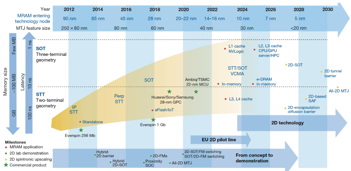
Figure 3. Technology Development Roadmap of MRAM [32].
