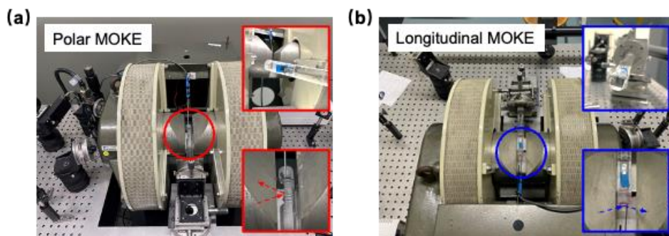
Figure 14. The MOKE system used in this work.
