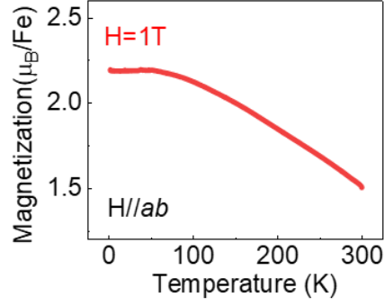
Figure 24. The in-plane M-T curve for 4 nm Fe 4 GeTe 2 at H=1T.
