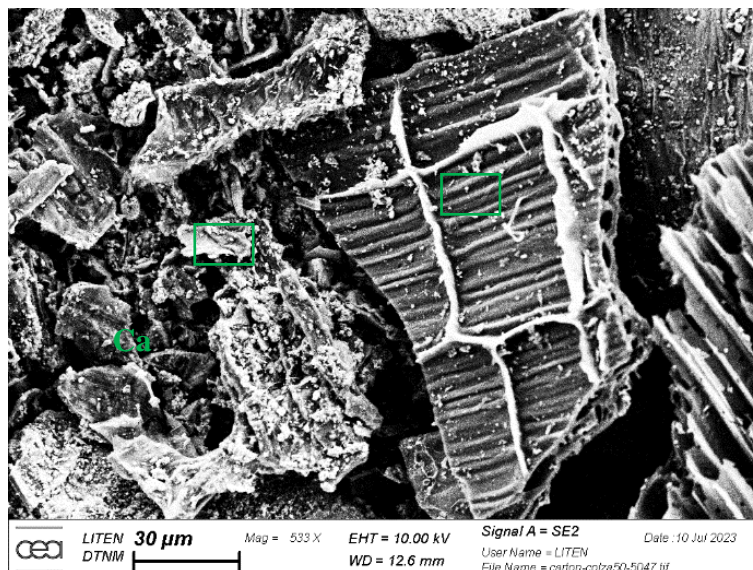
Figure 43: SEM observations of the char from co-pyrolysis at 800°C of 50/50 wt.% Cardboard + Colza straw mixture
