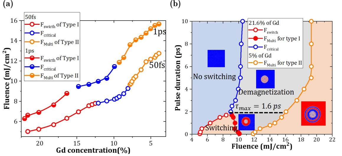
Figure 6.6: (a): F_{\text{switch}} for type-I, F_{\text{critical}} and F_{\text{multi}} for type-II as a function of Gd concentration for 50 fs and 1 ps laser pulse, respectively. (b): F_{\text{switch}} and F_{\text{multi}} for type-I and F_{\text{critical}} for type-I, but pulse duration is above maximum value to get switching ( \tau_{\max} = 1.6 ps) for 21.6% of Gd; and F_{\text{multi}} for type-II, as a function of pulse duration.
