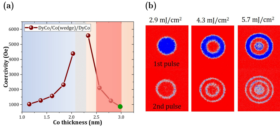
Figure 5.17: Single switching in Dy 35 Co 65 (4 nm)/Co(2 nm, wedge)/Dy 35 Co 65 (4 nm) tri-layer. The light red color shows the region of Co thickness ( 2.41 \text{ nm} < t_{\text{Co}} < 3.02 \text{ nm} ) where single shot switching occurs; (b) AOS results after each 50 fs laser pulse with different fluences, where t_{\text{Co}} = 2.98 \text{ nm} .
