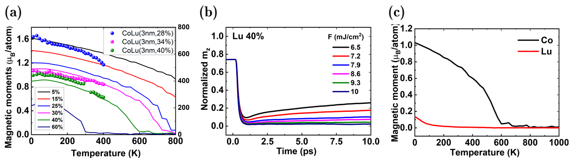
Figure 4.8: (a) Magnetic moment versus temperature for CoLu alloys with various concentrations. Sphere: experiments; lines: simulations; (b) Simulations of the Co demagnetization dynamics for the CoLu 40% alloy as a function of laser power. (c) Simulations of the magnetic moment versus temperature for both Co and Lu subnetworks in the case of CoLu 40% .
