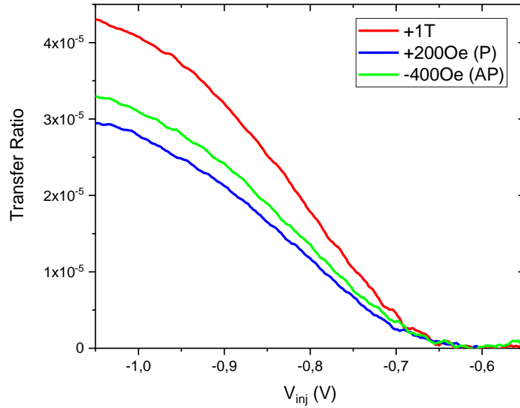
Figure IV.52: Transfer Ratio of a Co_{17.5}Cu_{82.5}(5) as a function of injection voltage at 35K for three different magnetic configurations of the MTT: saturated MTT (+1T), parallel configuration for MTJ electrodes (+200Oe), antiparallel configuration of electrodes (-400Oe). P and AP states are associated with minimum and maximum resistance values respectively (see Fig. IV.47).
