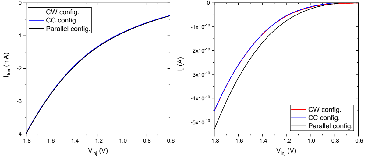
Figure IV.19: Tunnel current (left panel) and collected current (right panel) as a function on injected voltage for a \text{Co}_{50}\text{Al}_{50}(5) MTT at 50K in the three magnetic configurations (clockwise, counterclockwise and parallel).
