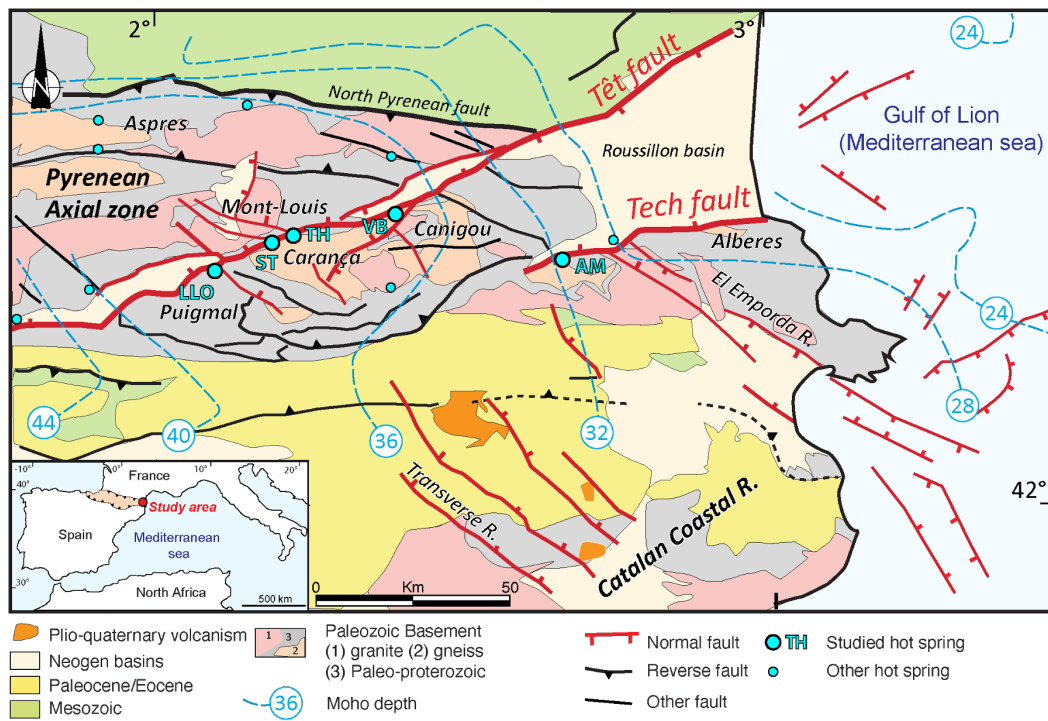
Figure 1: Structural map of Eastern Pyrenees modified after Taillefer et al. (2021). The name of the hot spring clusters studied are indicated: Llo, St-Thomas-les-Bains/Prats-Balaguer (ST), Thuès-les-Bains/Canaveilles (TH), Vernet-les-Bains (VB), Amélie-les-Bains (AM). Moho depth isocontours are modified from Goula et al. (1999), Mauffret et al. (2001) and Nercessian et al. (2001).
