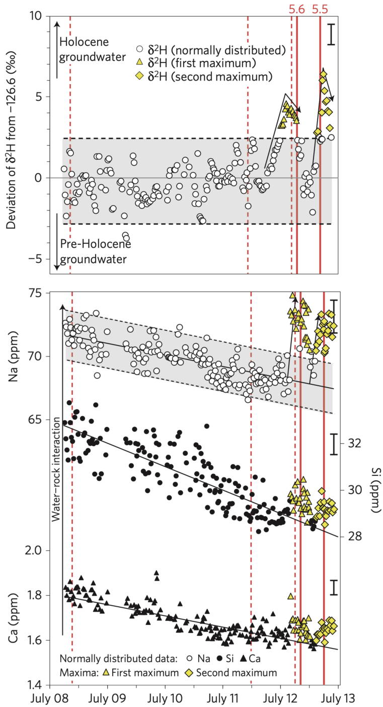
Figure 1.13: Time series for Ca, Si, and Na concentrations and \delta^2\text{H} deviation from -126.6 ‰ of groundwater from 2008 to 2013 collected at borehole HA-01. Earthquakes are shown by solid ( M > 5 ) and dashed ( M < 5 ) red lines. Normally distributed data are shown by open circles ( \delta^2\text{H} , \delta^{18}\text{O} , Na), black circles (Si) and triangles (Ca) with mean values (thin solid line) and 2\sigma envelopes (thin dashed lines and shading). Pre-seismic maxima are shown by yellow symbols. Pre- and co-seismic changes are shown by arrows. Analytical errors are shown above the top right of the data. Figure modified from Skelton et al. (2014).
