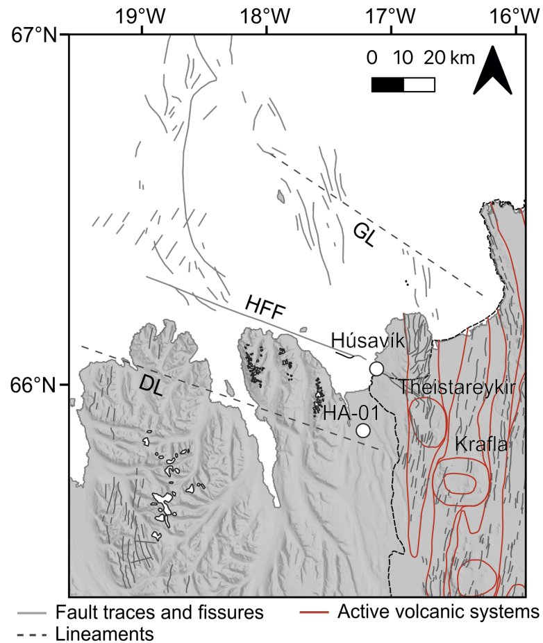
Figure 1.11: Main tectonic elements and volcanic centres near HA-01. DL refers to the Dalvík Lineament, HFF to Húsavík-Flatey Fault, and GL to Grímsey Lineament.
