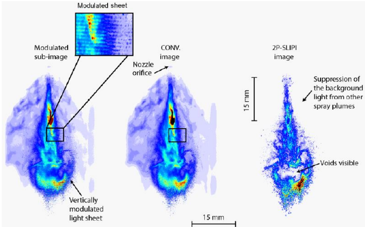
Figure 2-5 Instantaneous image of fluorescence in a spray. By recording two spatially modulated images in a very short time interval (typically a few hundred ns) and vertically shifting the modulations between the two images, it is possible to reconstruct an image in which the light background linked to multiple scattering is suppressed.
