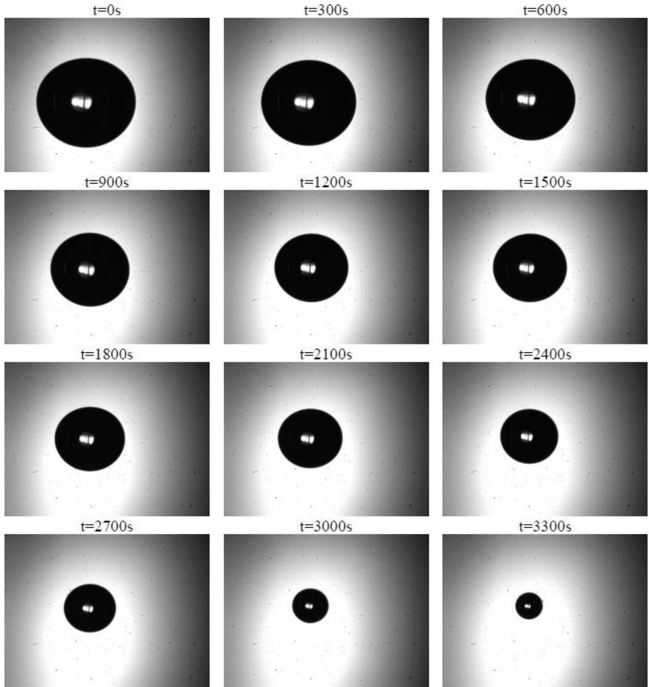
Figure 5-27 Case of a round water droplet evaporating in air at T_{\infty} = 20^{\circ}\text{C} and H=42\% (Relative Humditiy). The initial diameter of the drop is 2.0 mm.
