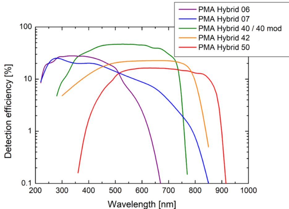
Figure 3-3 Spectral response of different type of PMA Hybrid
