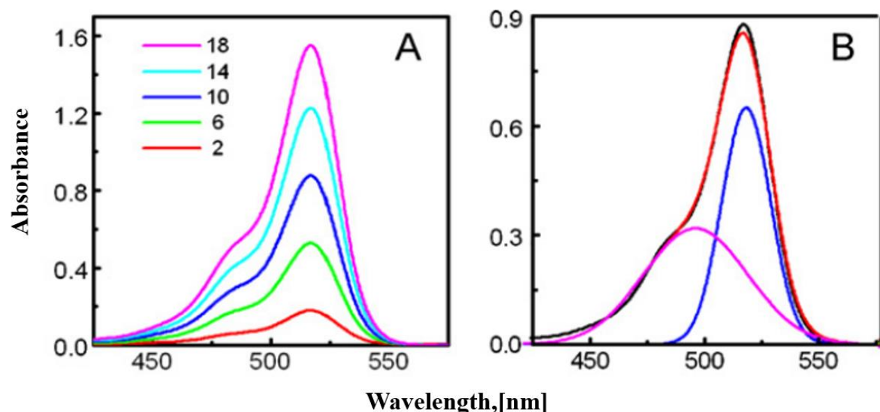
Figure 5-16 (A) Absorption spectra of EY dissolved into water at different concentrations (in \mu\text{M} , mentioned inside the figure). (B) Resolved absorption spectra of 10 \mu\text{M} EY in \text{H}_2\text{O} (purple for the dimer and blue for the monomer). The red and black lines represent the reconstituted and original spectra of EY respectively. Figure extracted from Chakraborty et al. (2011) [26].
