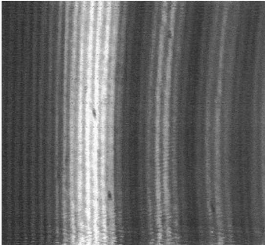
Figure 2-8 Standard rainbow pattern obtained from a single droplet in a water spray. Reprinted from [46]
