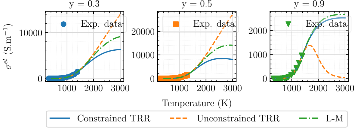
Figure 3.22: Optimization results obtained with three methods : constrained TRR, unconstrained TRR and L-M. The constrained TRR was performed with the following bounds : H \in [0.5 - 1.5] eV, \frac{S}{k} \in [2 - 12] , E_m(Pu) \in [0.04 - 0.5] eV, E_m(U) \in [0.06 - 0.5] eV.
