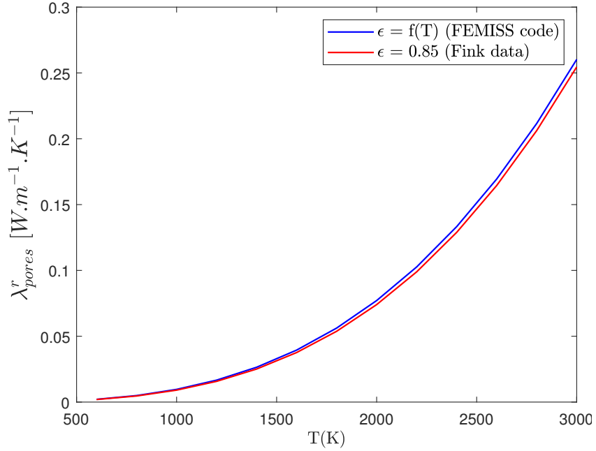
Figure 2.4: Variation with temperature of thermal conductivity due to radiation across the pores, using a temperature-dependent emissivity model (FEMISS code) and a constant value (Fink [87])
