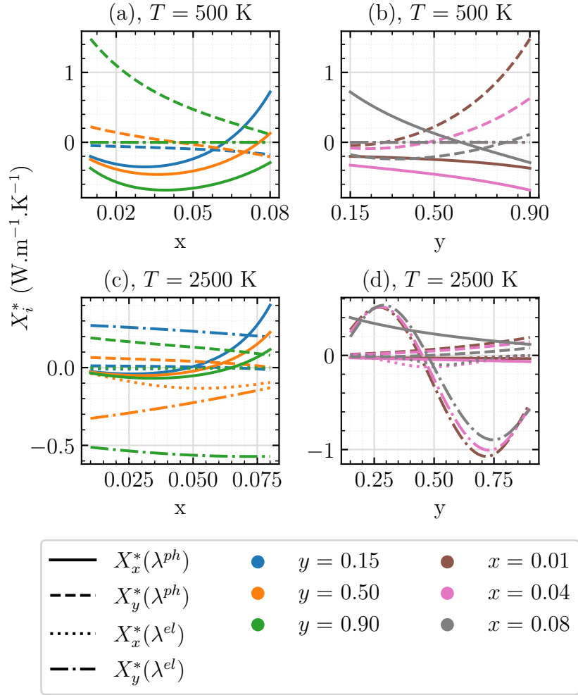
Figure 3.31: Comparison of the sensitivity coefficients of the electron and phonon terms on x and y . Their variations with x and y are plotted for T = 500 \text{ K} and T = 2500 \text{ K} at (a), (b) and (c), (d) respectively
