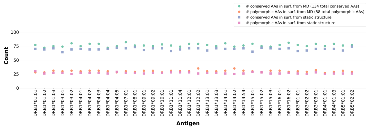
Figure S4: Conserved and polymorphic AA positions at surface in HLA antigen. Counting was made for MD and static PDB data (structures issued from the refinement process). A) Antigens from locus A ( \beta 2 -microglobulin not included). B) Antigens from locus B ( \beta 2 -microglobulin not included). C) Antigens from locus C ( \beta 2 -microglobulin not included). D) Antigens from locus DP. E) Antigens from locus DQ. F) Antigens from locus DR (chain encoded from gene DRA1 not included).
