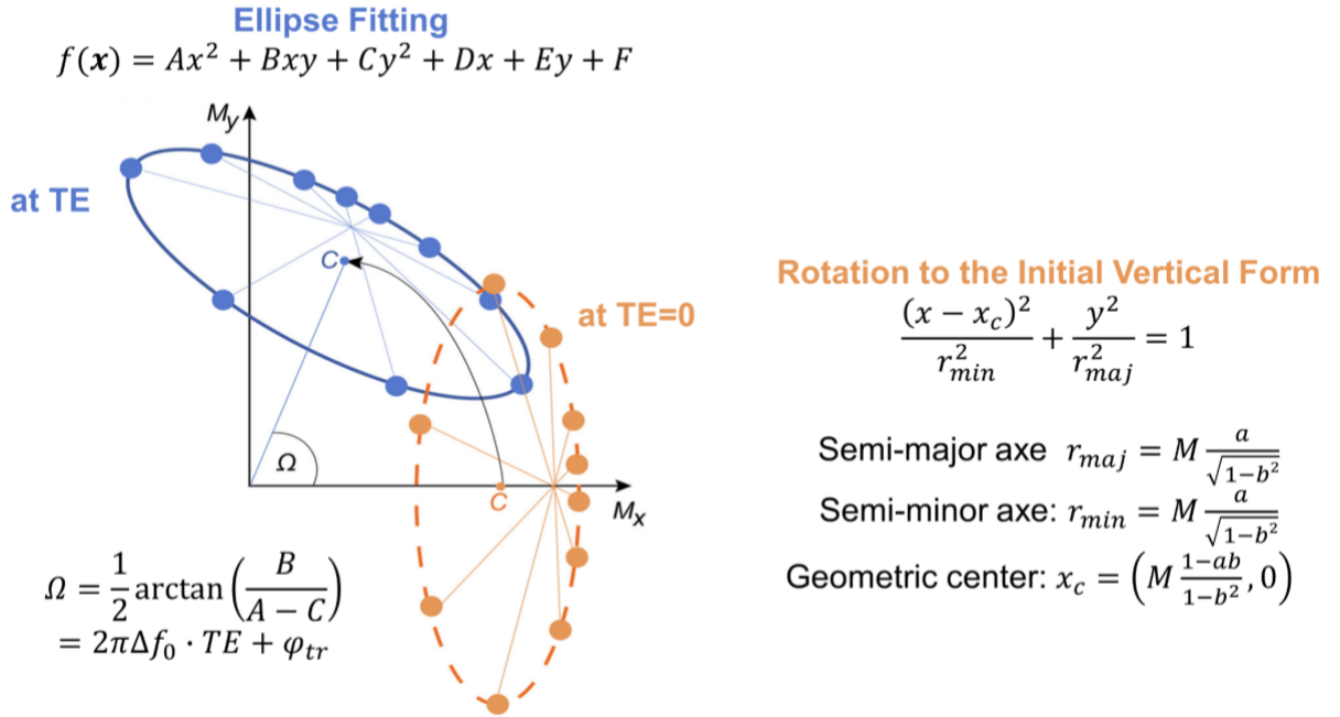
Figure 7. Adapted from Gavazzi et al. 2020 [97]. The complex bSSFP signal right after the RF excitation (at TE=0 s) defines a vertically-orientated ellipse (in orange). At TE, the ellipse rotates by an angle \Omega to form the blue ellipse. The measured phase-cycled bSSFP data points are depicted as colored dots. The geometry of the orange ellipse is linked to the three parameters of bSSFP signal (M, a and b), establishing three equations with three unknowns that can be solved.
